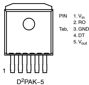
Figure 3. Pin Connections
