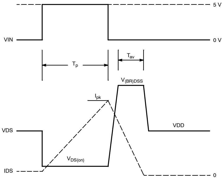
Figure 26. Inductive Load Switching Waveforms
