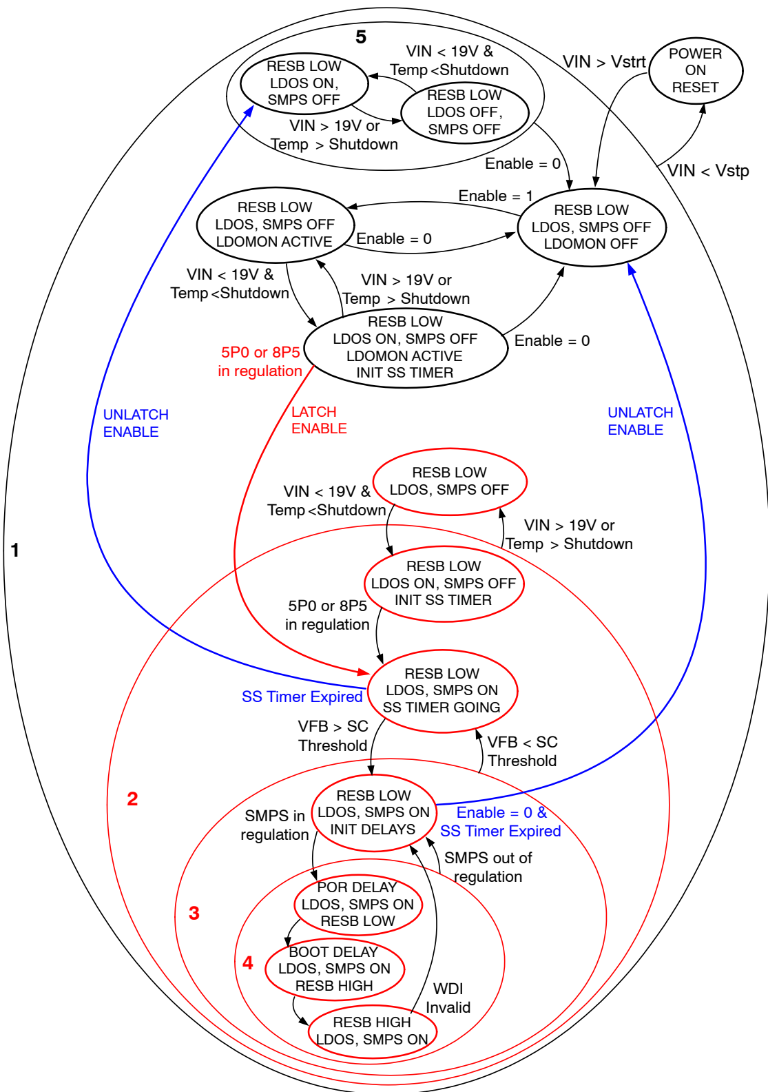
Figure 41. State Diagram
