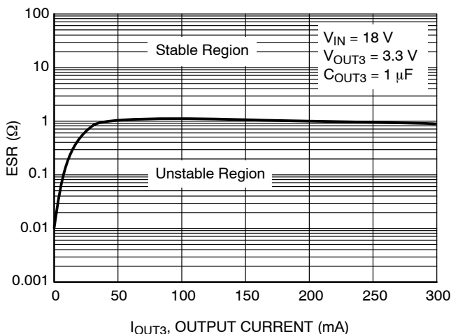
Figure 24. C_{OUT3} ESR Stability Region – 1 \mu F
