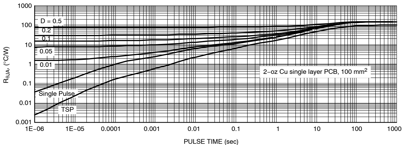
Figure 19. R_{\theta JA} vs. Duty Cycle
