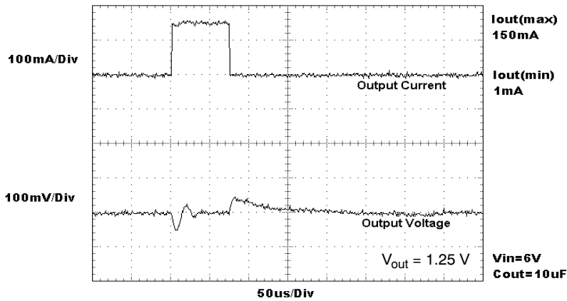
Figure 32. Load Transient Response (10 μF)
