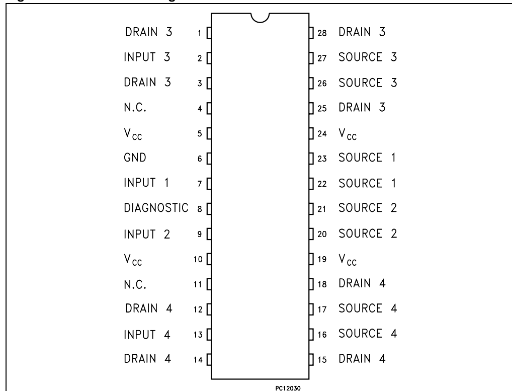
Figure 2. Connection diagram
