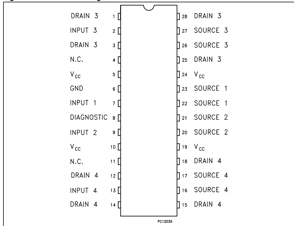
Figure 2. Connection diagram
