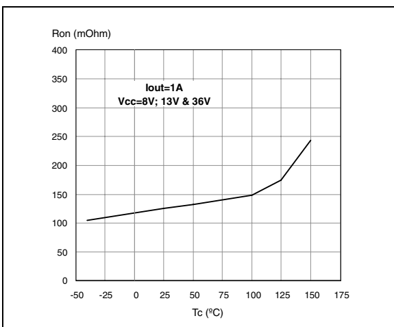
Figure 16. On-state resistance vs T_{case}
