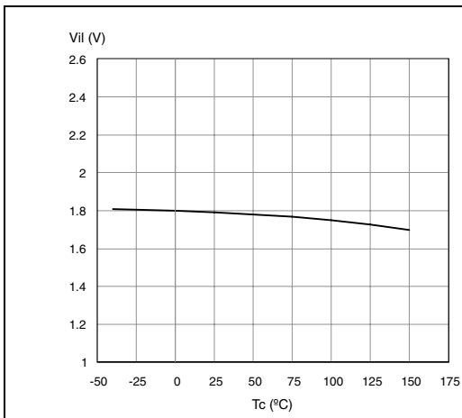
Figure 10. Input low level voltage
