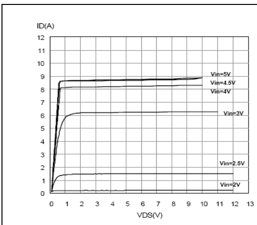
Figure 33. Output characteristics
