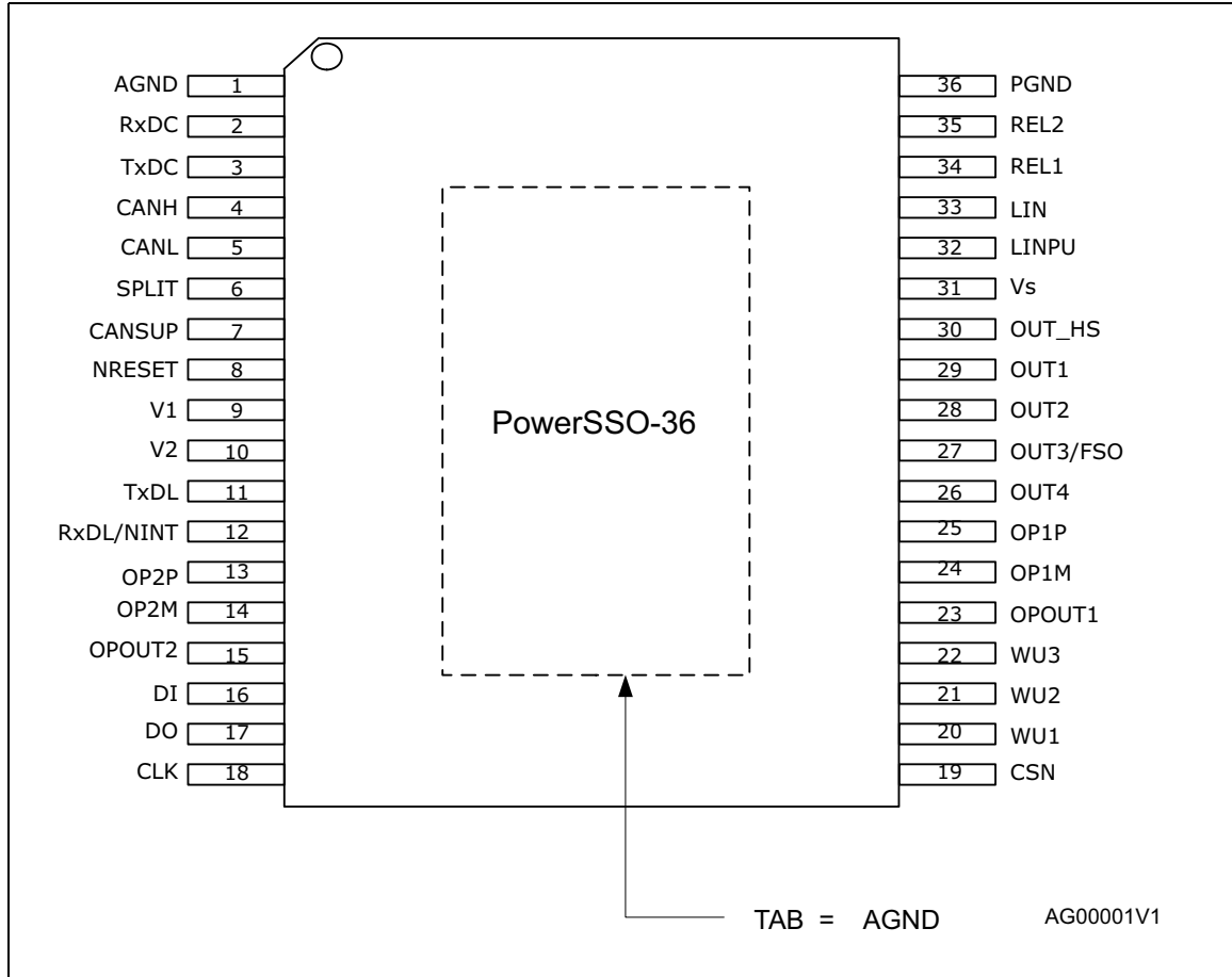
Figure 2. Pin connection (top view)
