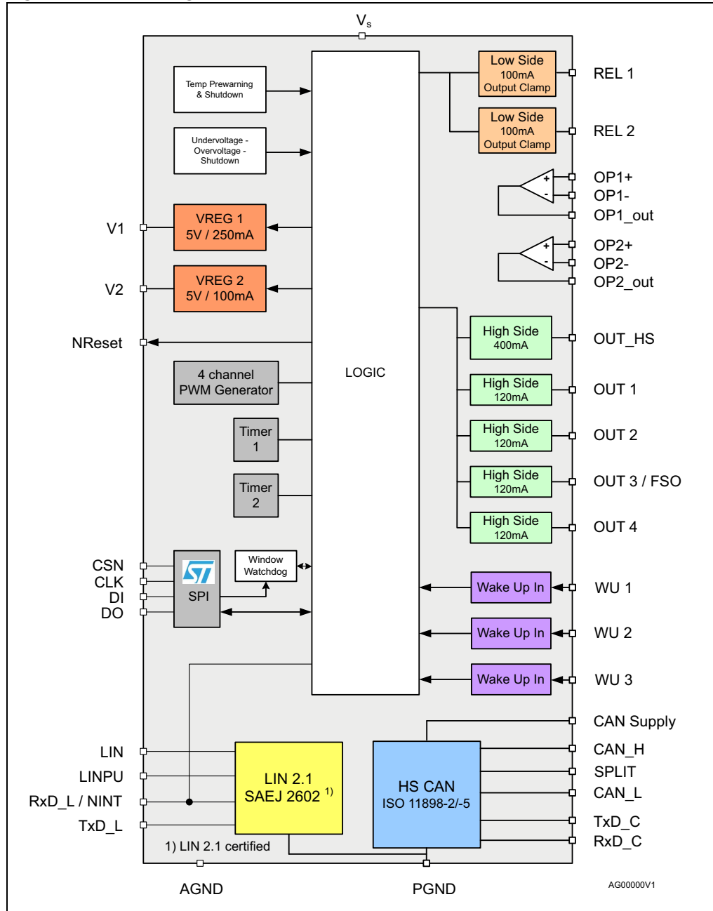
Figure 1. Block diagram
