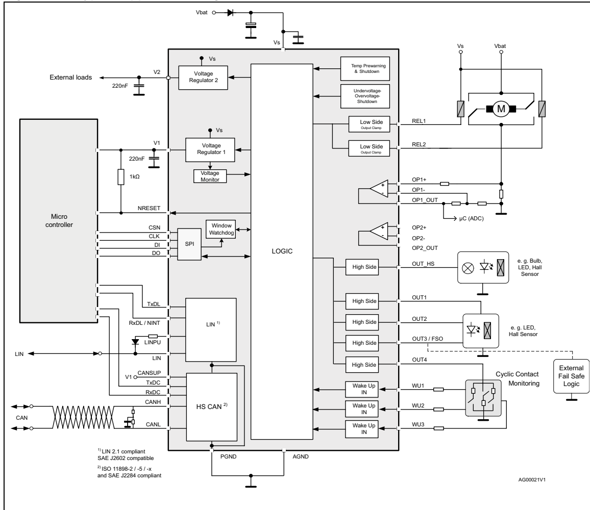
Figure 22. Typical application diagram
