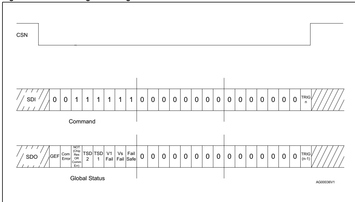
Figure 37. Write configuration register (1)
