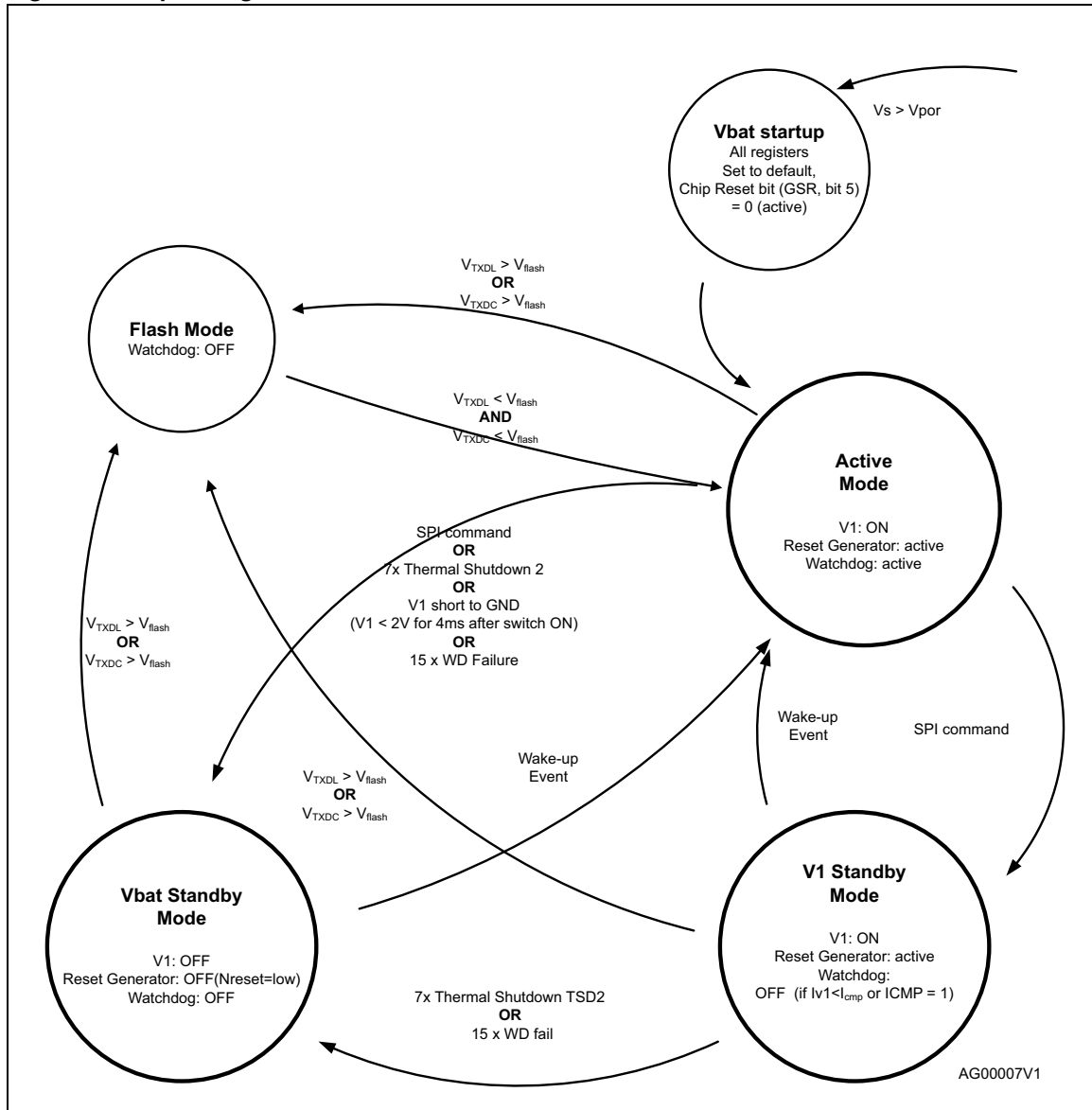
Figure 8. Operating modes
