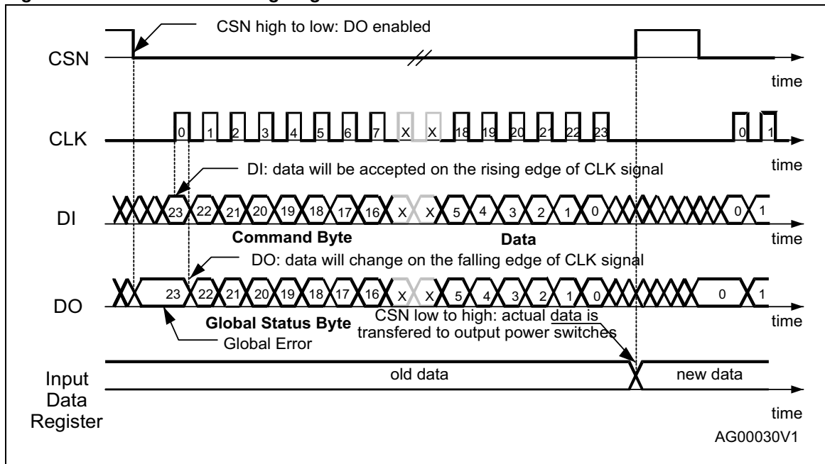
Figure 31. SPI – transfer timing diagram
