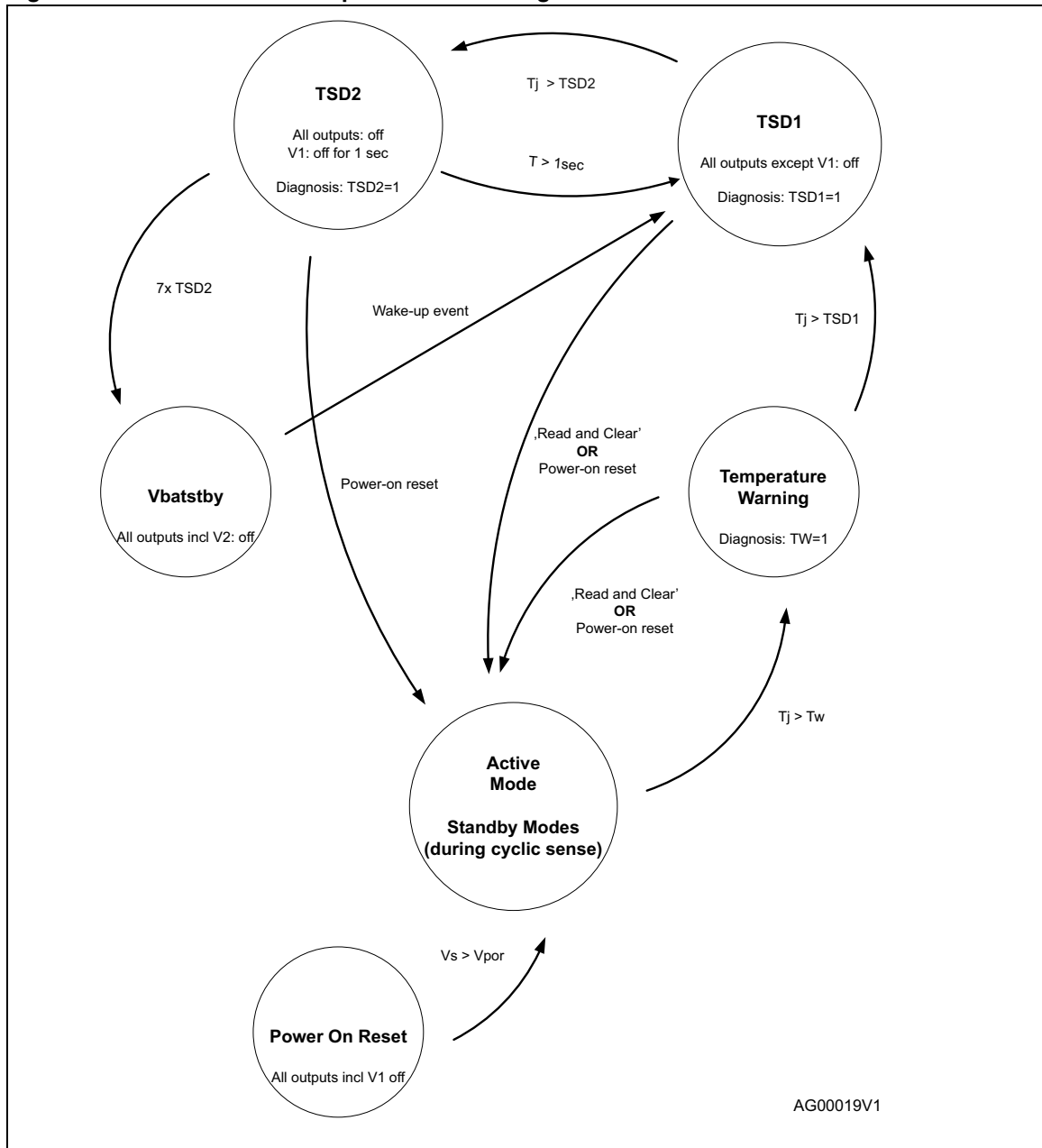
Figure 20. Thermal shutdown protection and diagnosis
