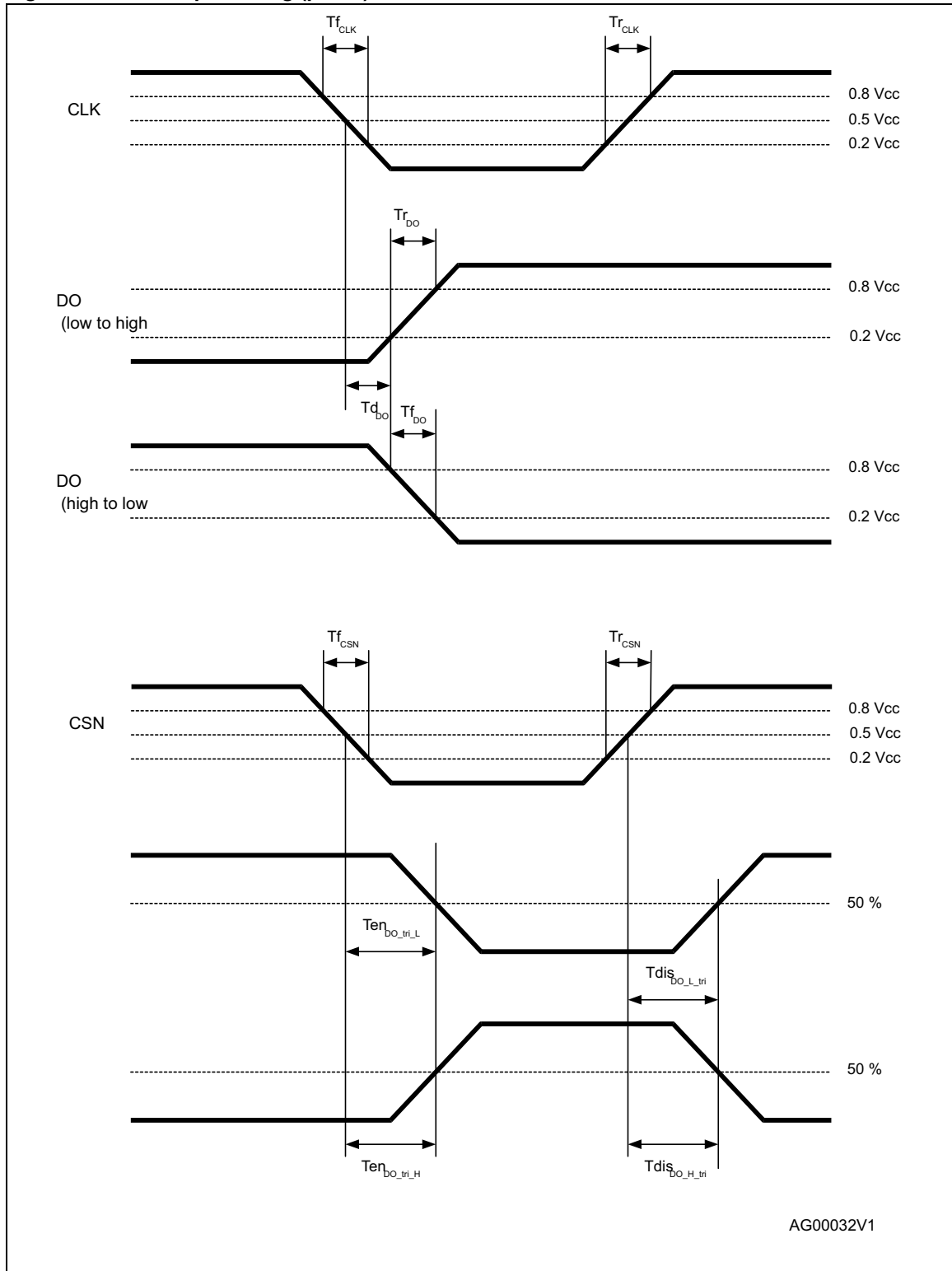
Figure 33. SPI output timing (part 1)
