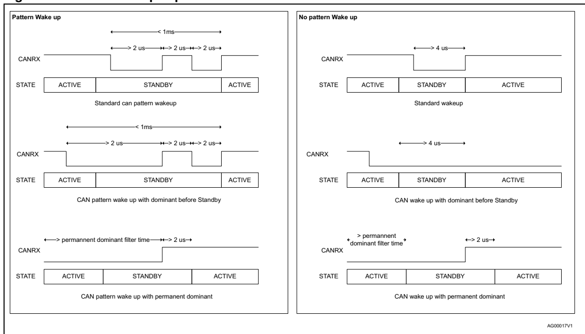
Figure 18. CAN wake up capabilities
