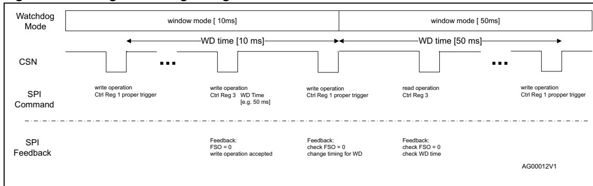
Figure 13. Change watchdog timing within window mode
