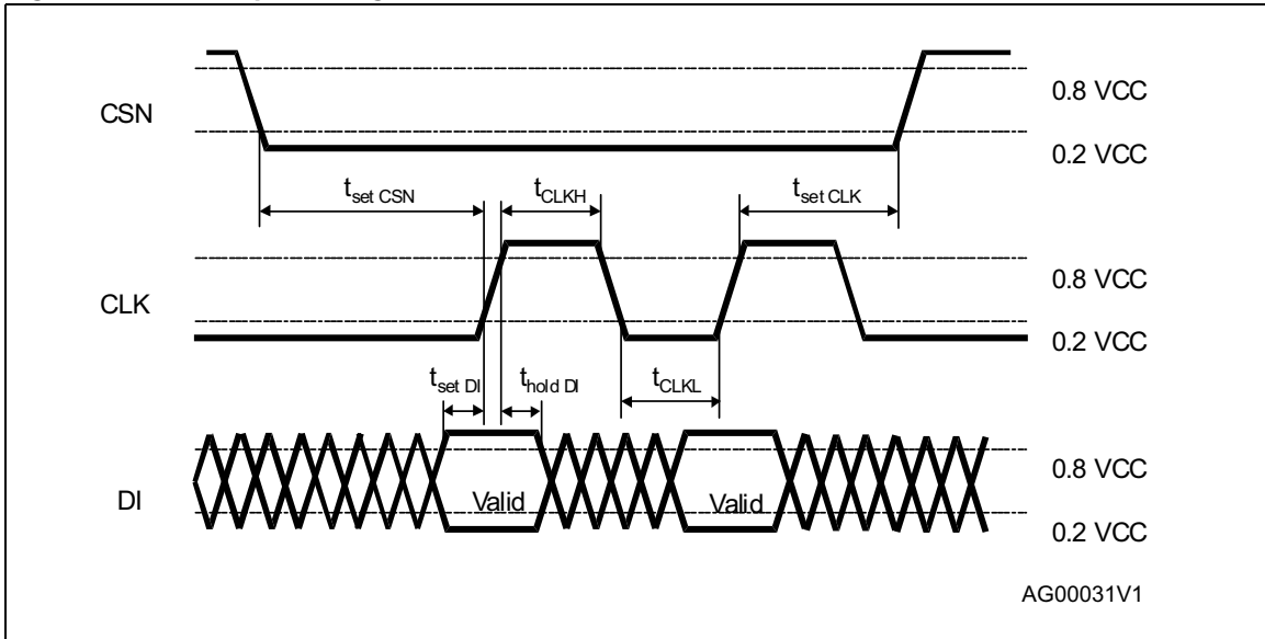
Figure 32. SPI - input timing
