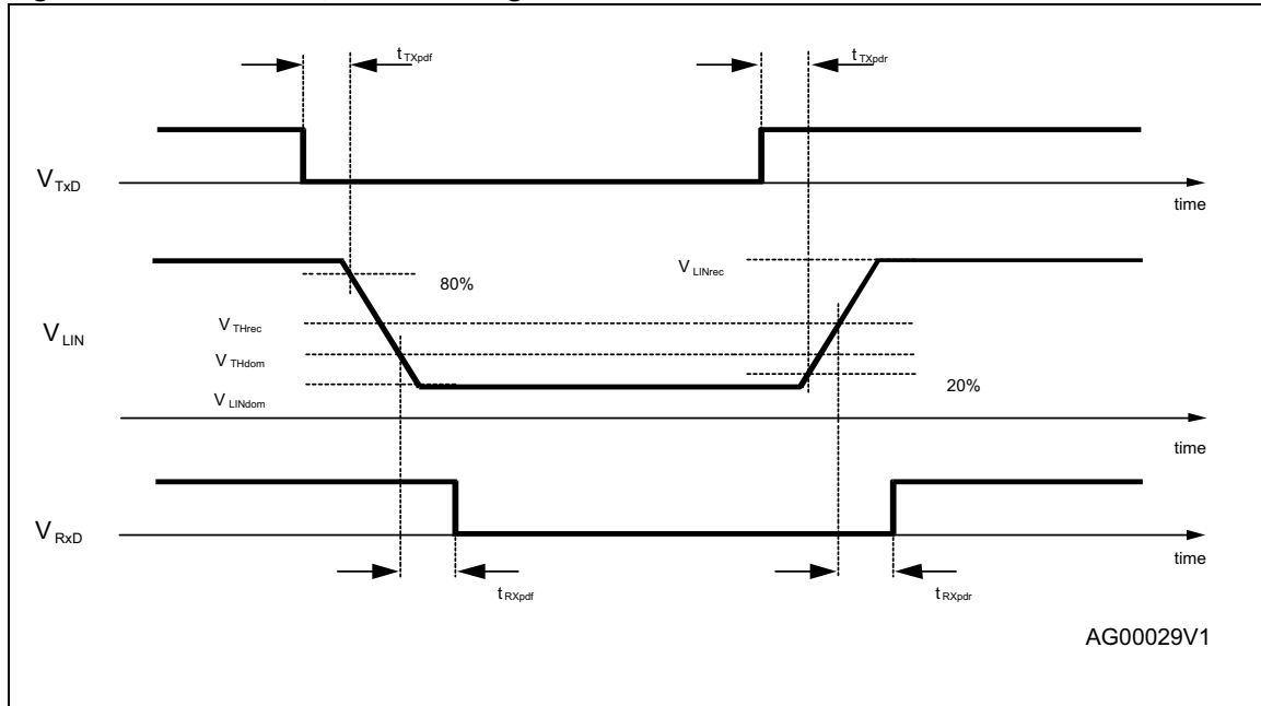
Figure 30. LIN transmit, receive timing
