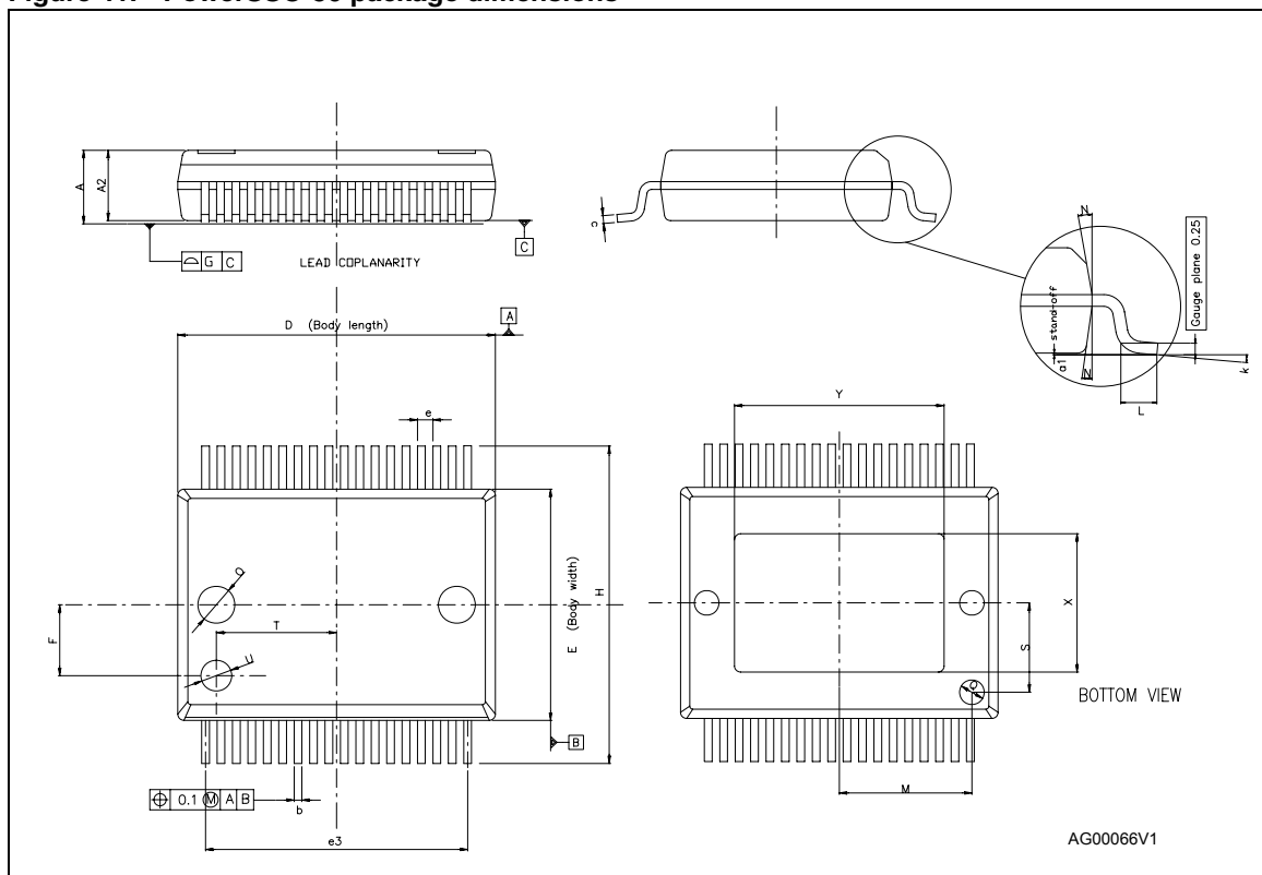
Figure 41. PowerSSO-36 package dimensions
