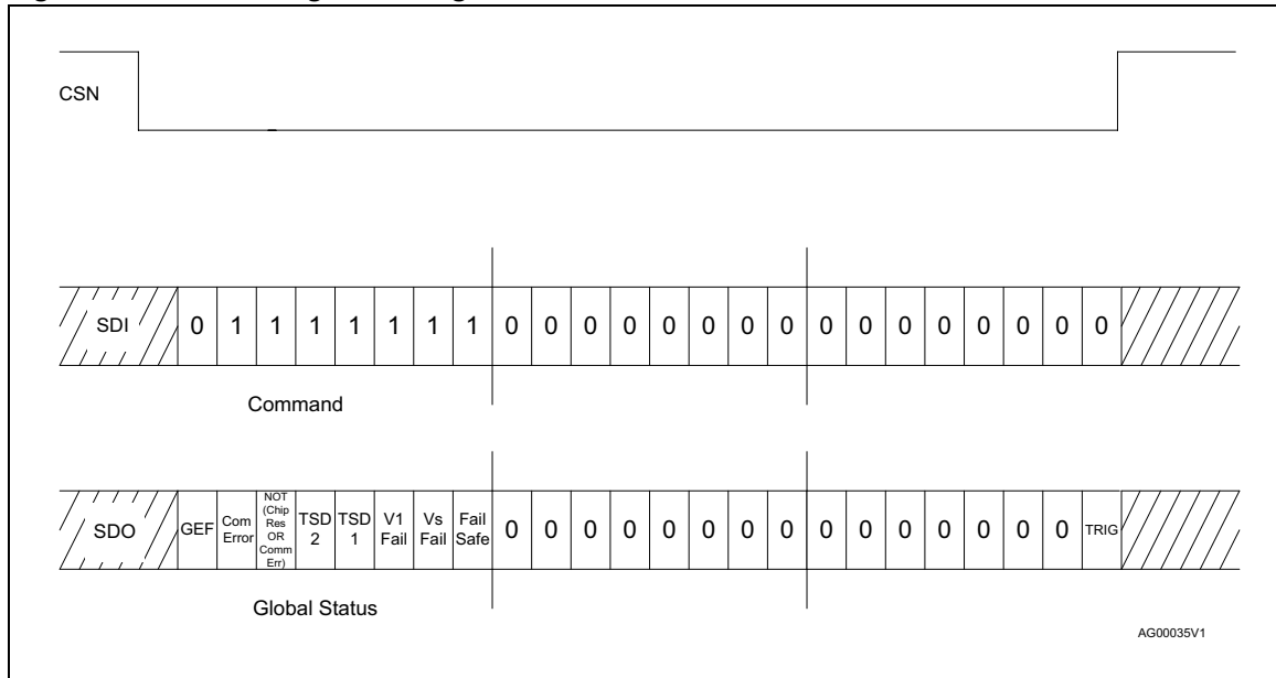
Figure 36. Read configuration register (1)
