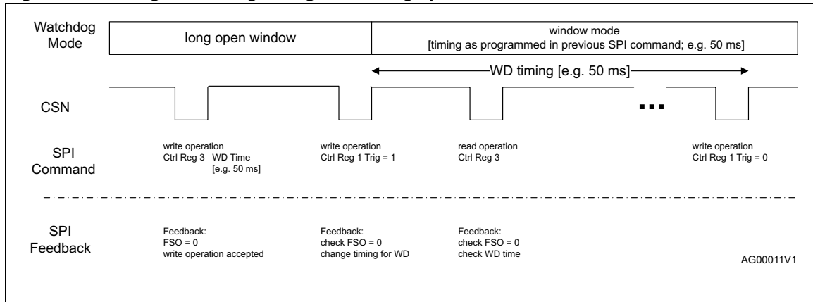
Figure 12. Change watchdog timing within long open window
