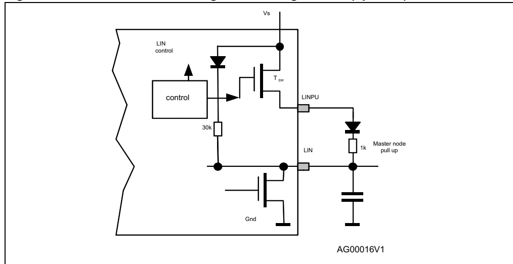
Figure 17. LIN master node configuration using LIN_PU (optional)
