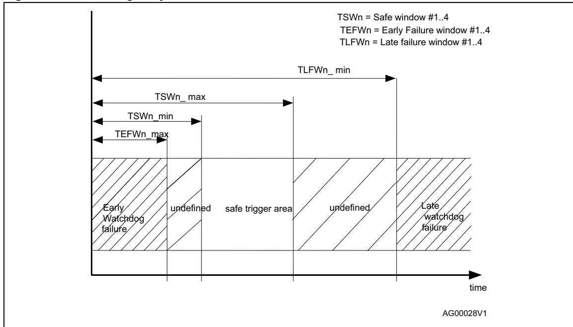
Figure 29. Watchdog early, late and safe windows
