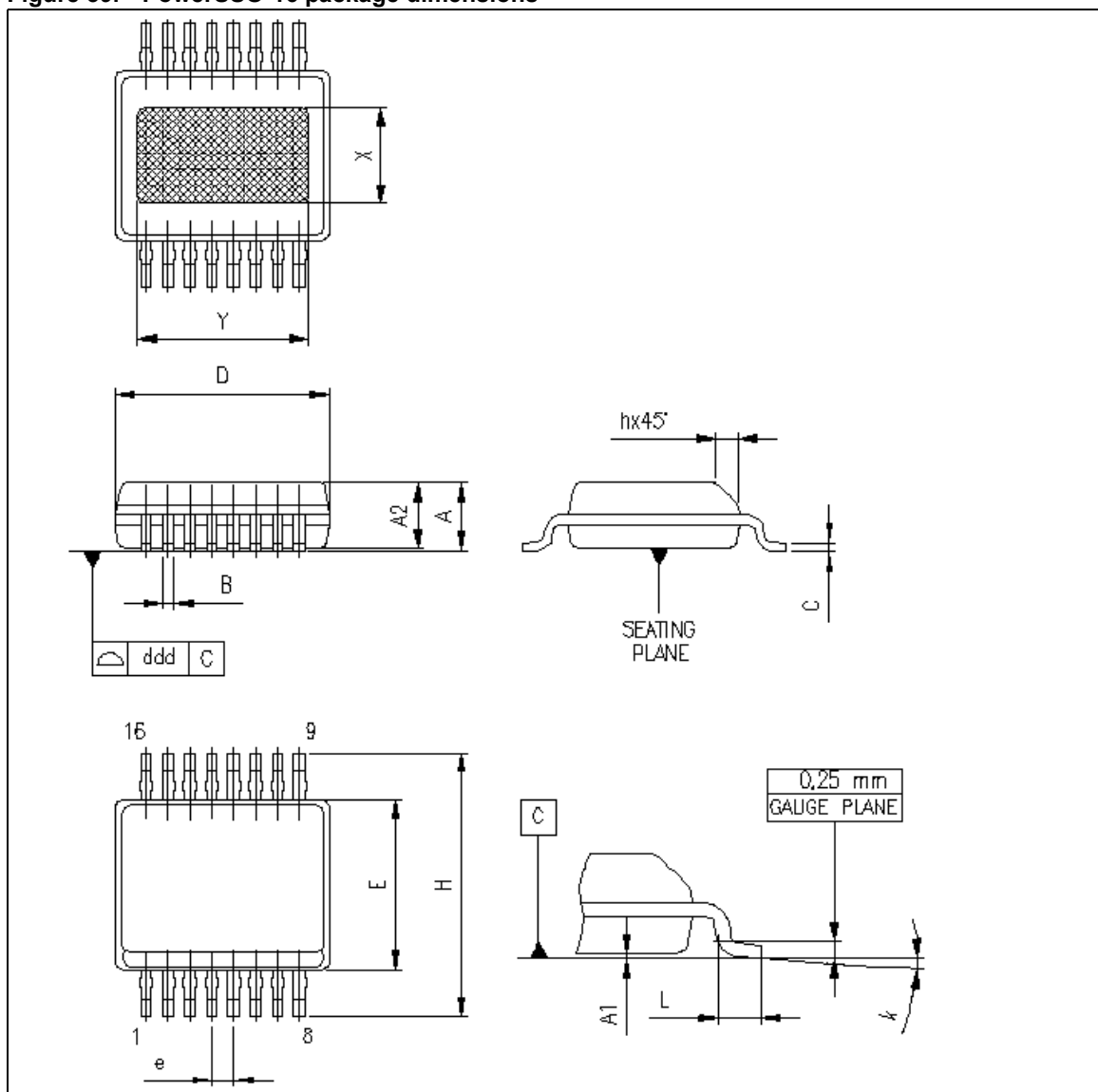
Figure 39. PowerSSO-16 package dimensions
