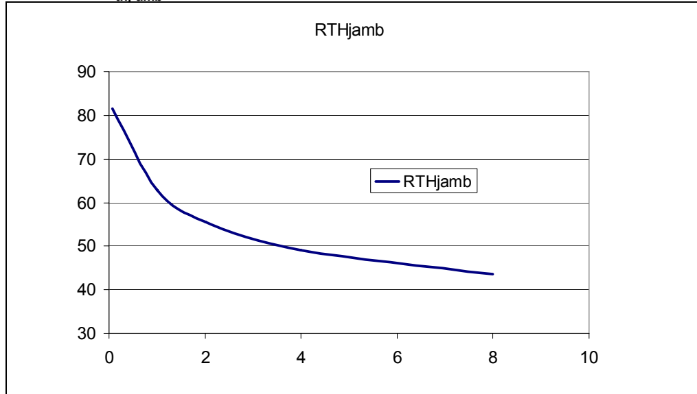
Figure 36. R_{thi-amb} vs PCB copper area in open box free air condition (one channel ON)
