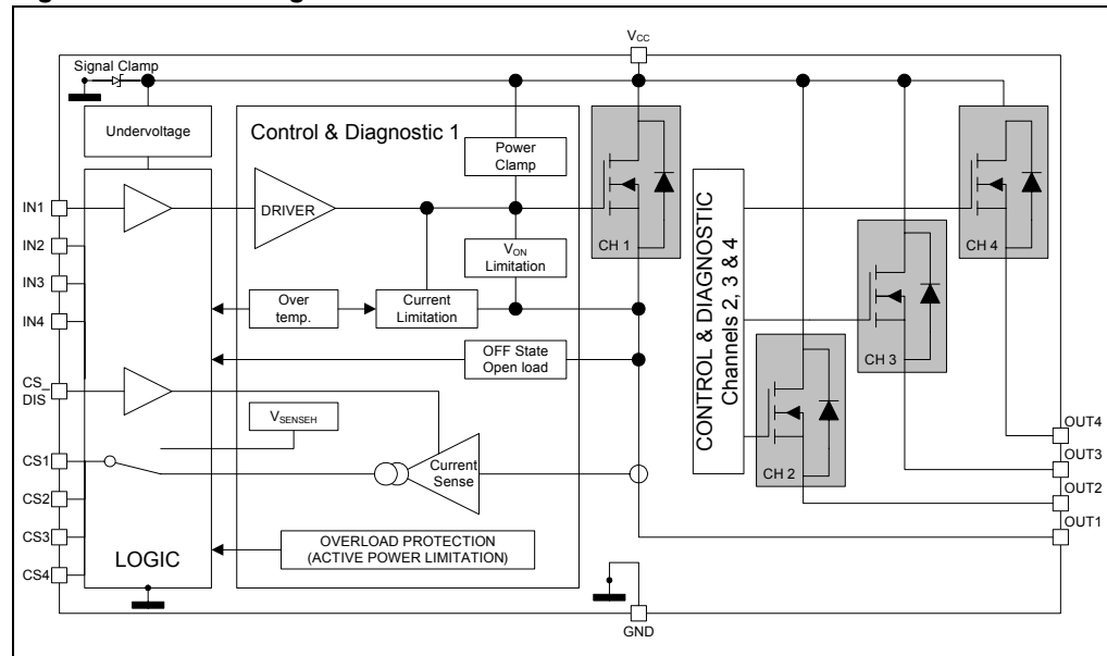
Figure 1. Block diagram
