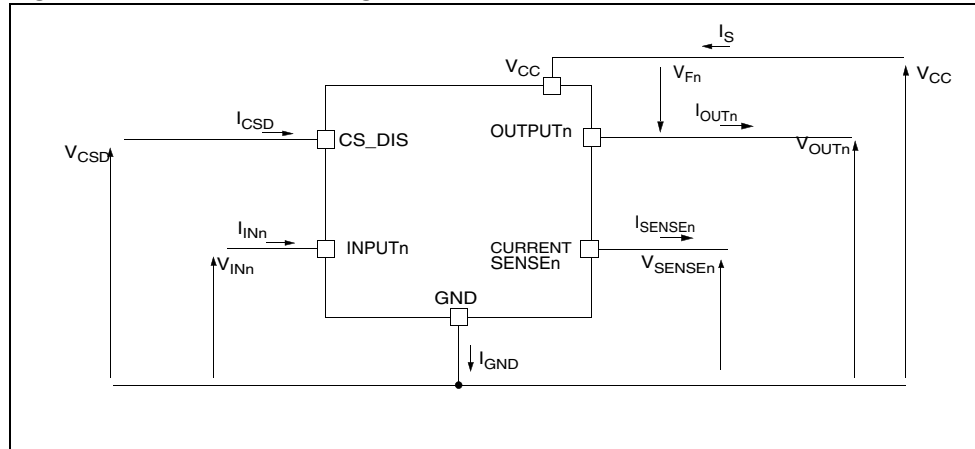
Figure 3. Current and voltage conventions
