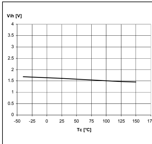
Figure 21. Input high-level voltage
