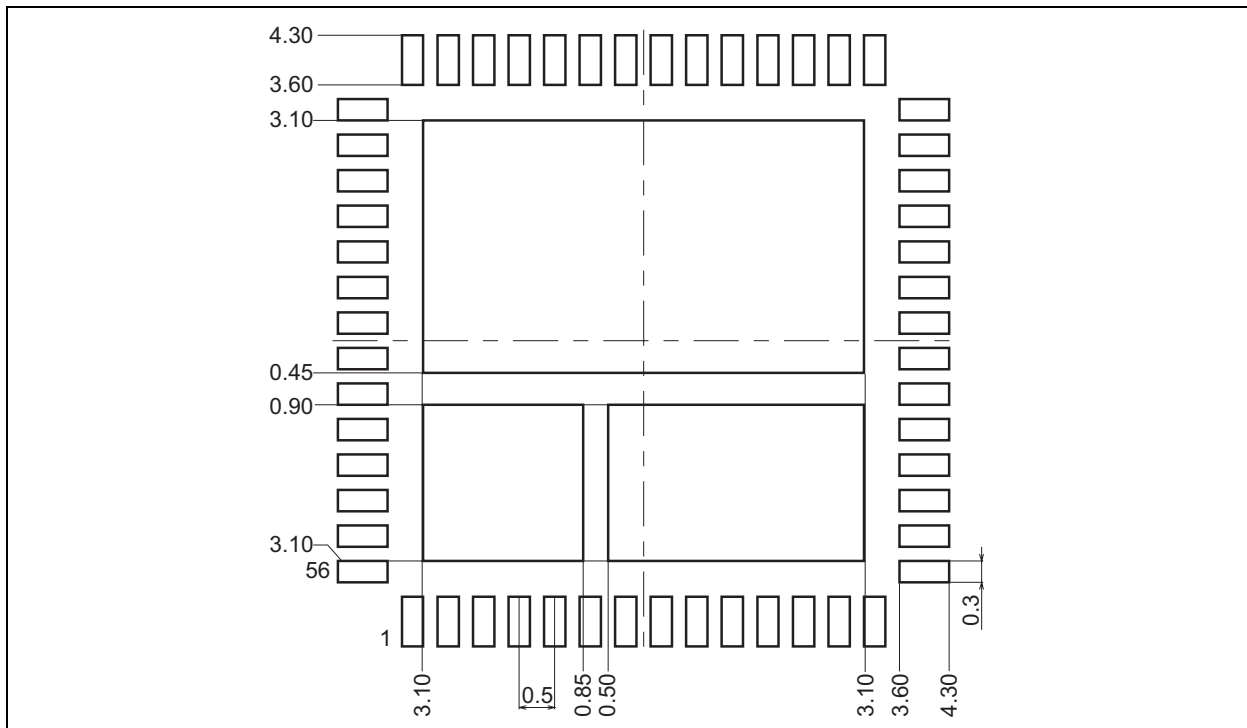
Figure 3 Footprint Example
