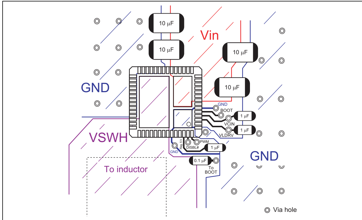
Figure 2 R2J20602NP PCB Layout Example (Top View)
