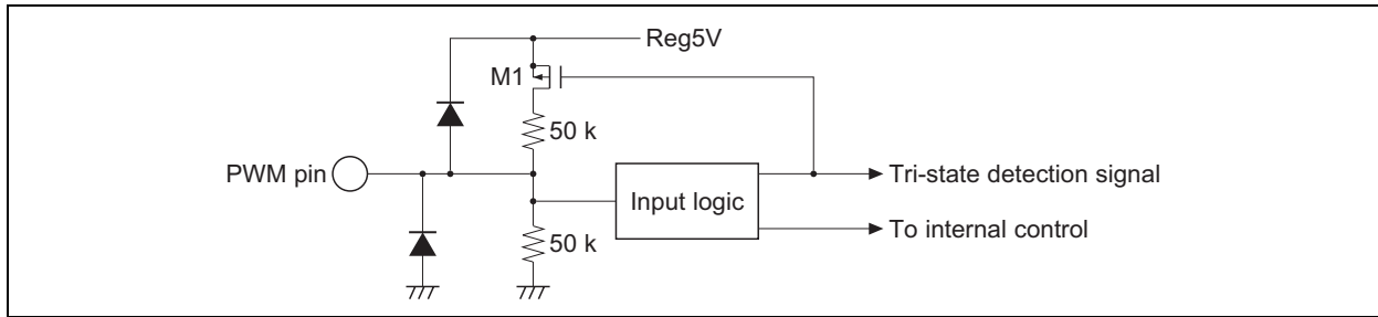
Figure 2 Equivalent Circuit for the PWM-pin Input
