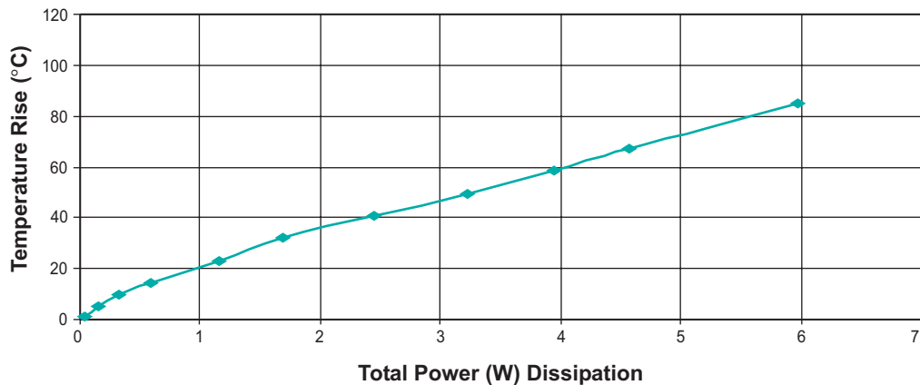
Temperature Rise vs. Power (W) Dissipation
