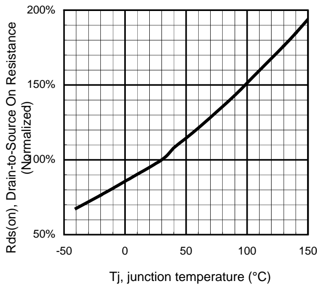
Figure 11 - Normalized R ds(on) (%) Vs T j (°C)
