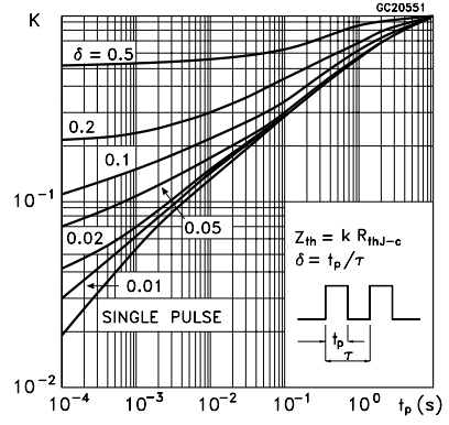
Thermal Impedance for SOT-223
