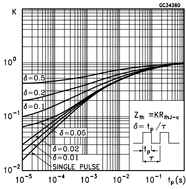
Thermal Impedance for DPAK/IPAK
