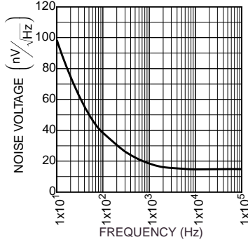
Voltage Noise
