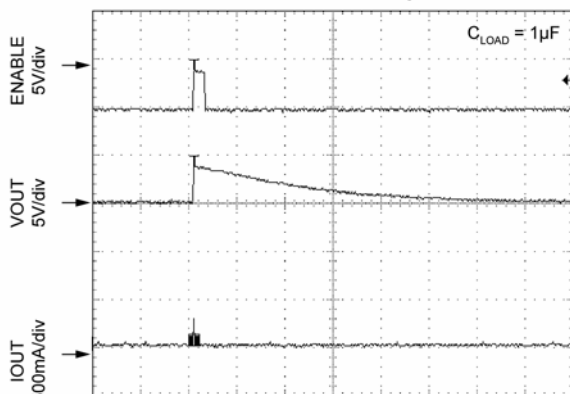
TIME 250µs/div
