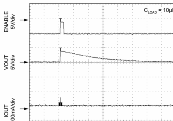
TIME 250µs/div
