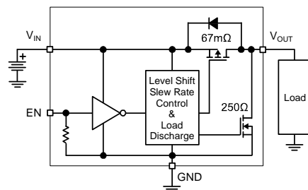
MIC94081 (ultra fast turn on with auto-discharge) MIC94083 (850μs soft-start with auto-discharge) MIC94085 (120μs soft-start with auto-discharge)
