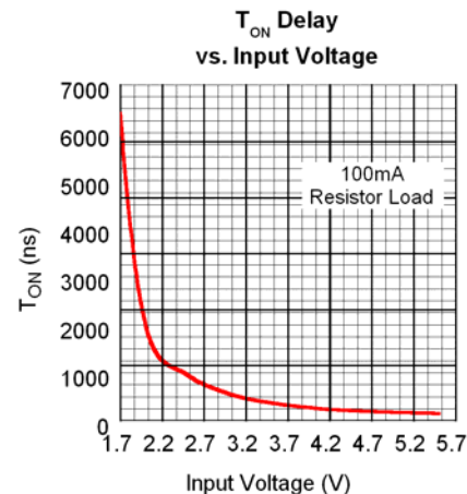
MIC94080/1
