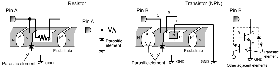
Pattern Diagram of Parasitic Element
