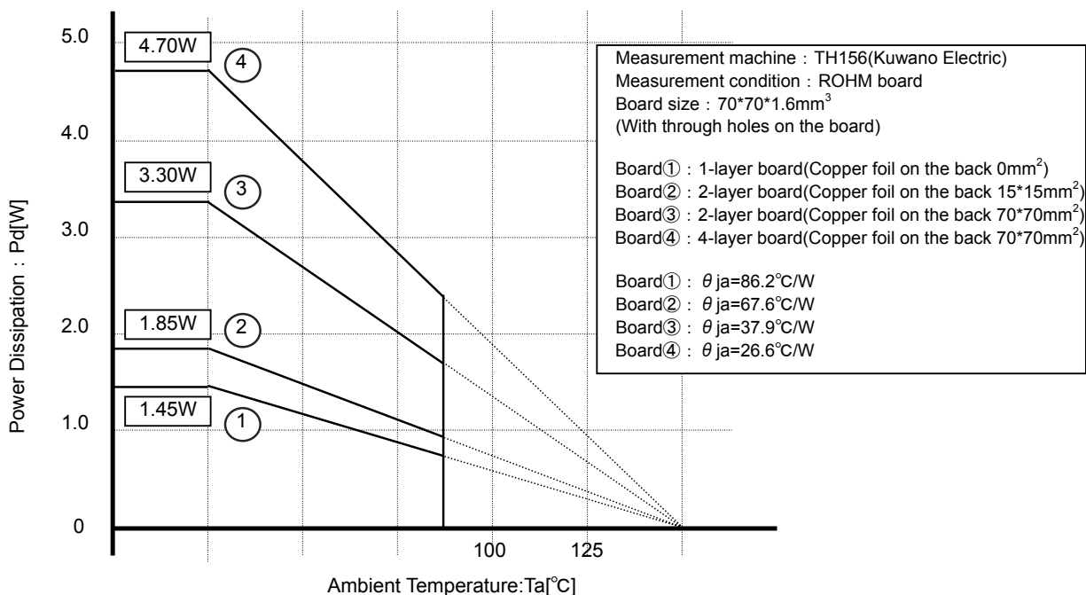
HTSSOP-B28 Derating Curve
