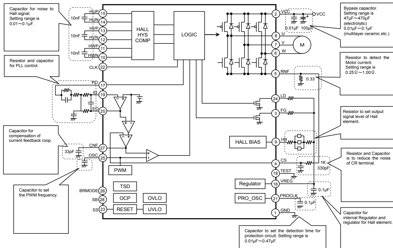
Block diagram & Application circuit diagram
