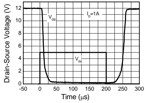
Switching Speed
