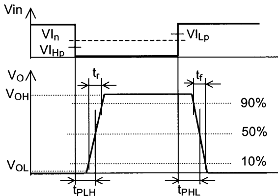
(1) Normal switching mode
