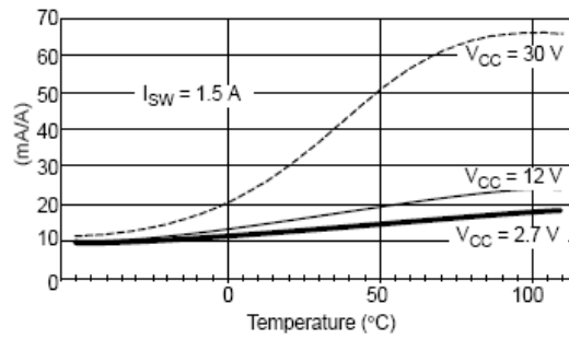
Figure 4. \Delta I_{CC}/\Delta V_{SW} vs. Temperature
