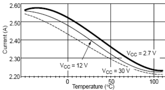
Figure 9. Current Limit vs. Temperature
