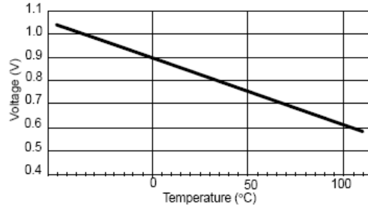
Figure 12. Shutdown Threshold vs. Temperature
