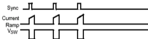
Figure 20. Timing Diagram of Sync and Shutdown
