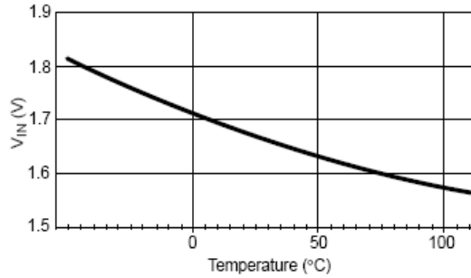
Figure 6. Minimum Input Voltage vs. Temperature
