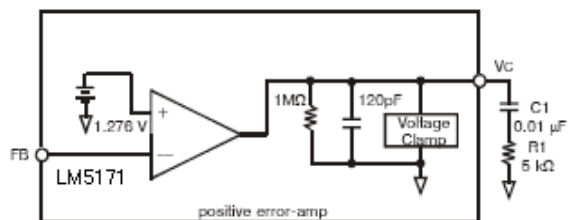
Figure 21. Error Amplifier Equivalent Circuit
