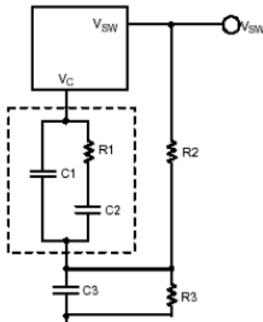
Figure 30. Technique for Increasing Slope Compensation
