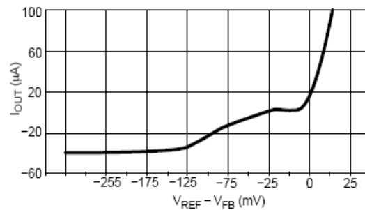
Figure 18. Error Amplifier I_{OUT} vs. V_{FB}
