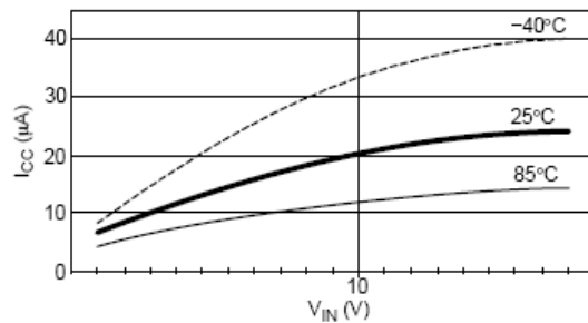
Figure 15. I_{CC} vs. V_{IN} During Shutdown
