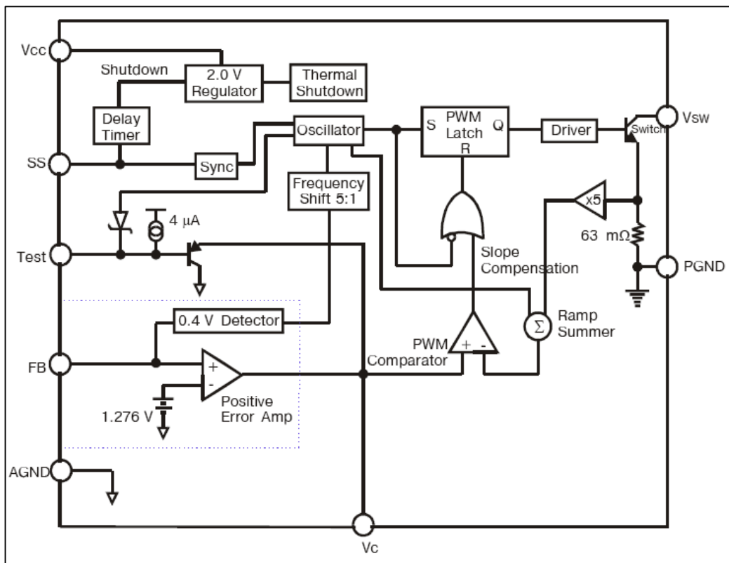
Figure 2. Block Diagram
