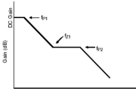
Figure 24. Bode Plot of the Compensation Network Shown in Figure 23.
