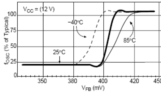
Figure 8. Switching Frequency vs. V_{FB}
