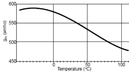
Figure 16. Error Amplifier Transconductance vs. Temperature
