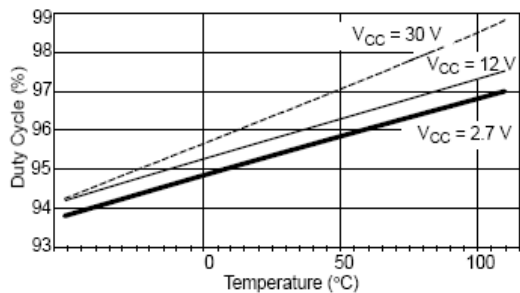
Figure 10. Maximum Duty Cycle vs. Temperature
