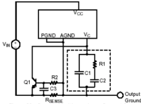
Figure 29. Current Limiting using a Current Sense Resistor
