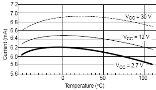
Figure 3. I_{CC} (No Switching) vs. Temperature
