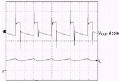
Figure 27. Typical Output Voltage Ripple
