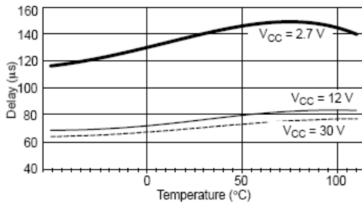
Figure 13. Shutdown Delay vs. Temperature
