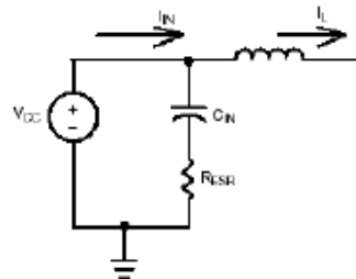
Figure 26. Boost Circuit Effective Input Filter
