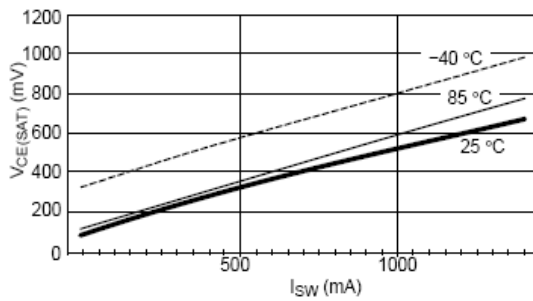
Figure 5. V_{CE(SAT)} vs. I_{SW}
