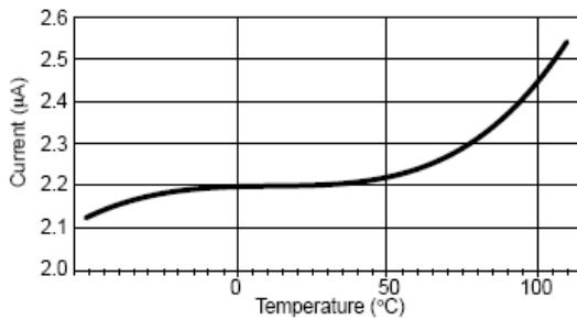
Figure 17. Switch Leakage vs. Temperature
