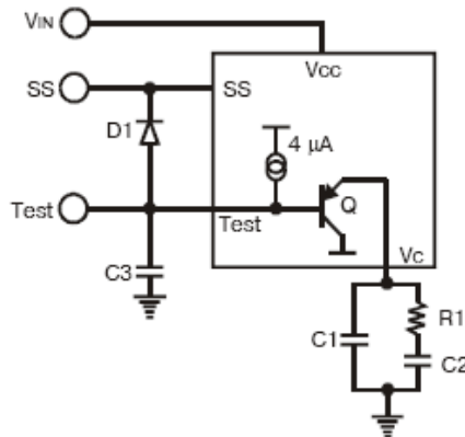
Figure 31. Soft Start
