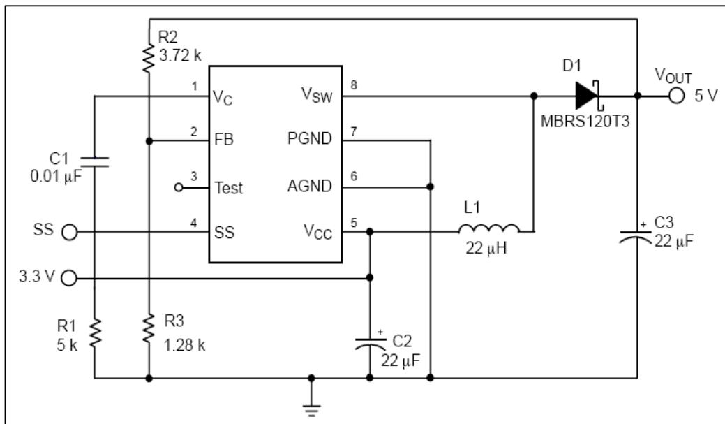
Figure 1. Application Circuit
