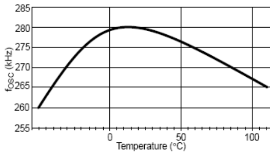
Figure 7. Switching Frequency vs. Temperature
