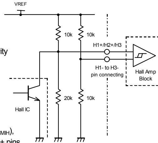
Figure2: Hall IC application
