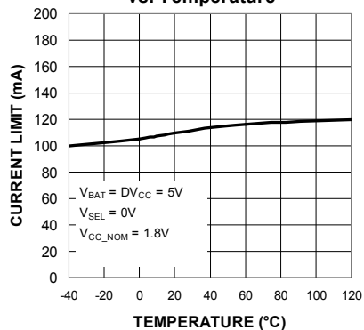
Current Limit V_{CC} vs. Temperature
