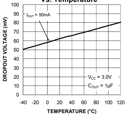
LDO Dropout vs. Temperature
