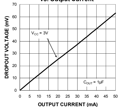
LDO Dropout vs. Output Current
