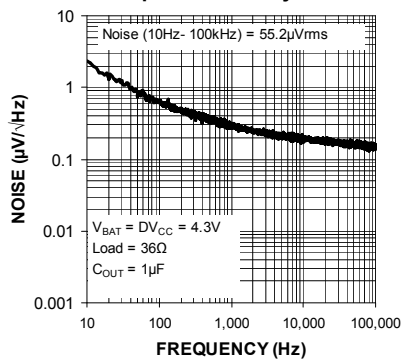
LDO Output Noise Spectral Density
