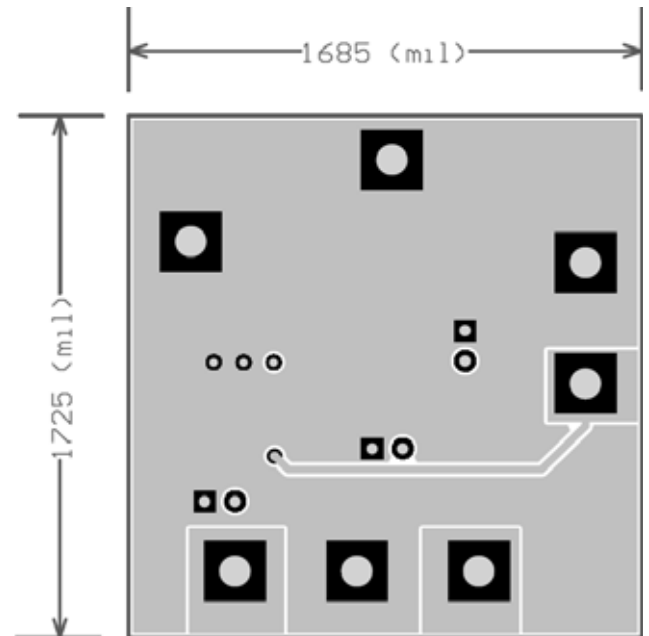
Figure 3. MIC47300 EVB Bottom Layer
