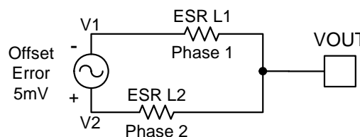
Figure 10 – Error Amplitude
