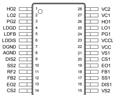
PW PACKAGE (Top View)
