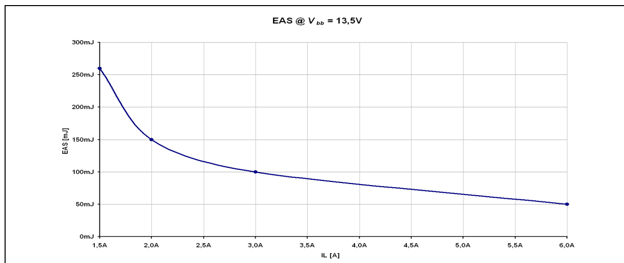
Figure 9 Maximum Energy Dissipation Single Pulse, T_{j,Start} = 150^\circ C
