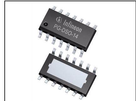
PG-DSO-14-33
