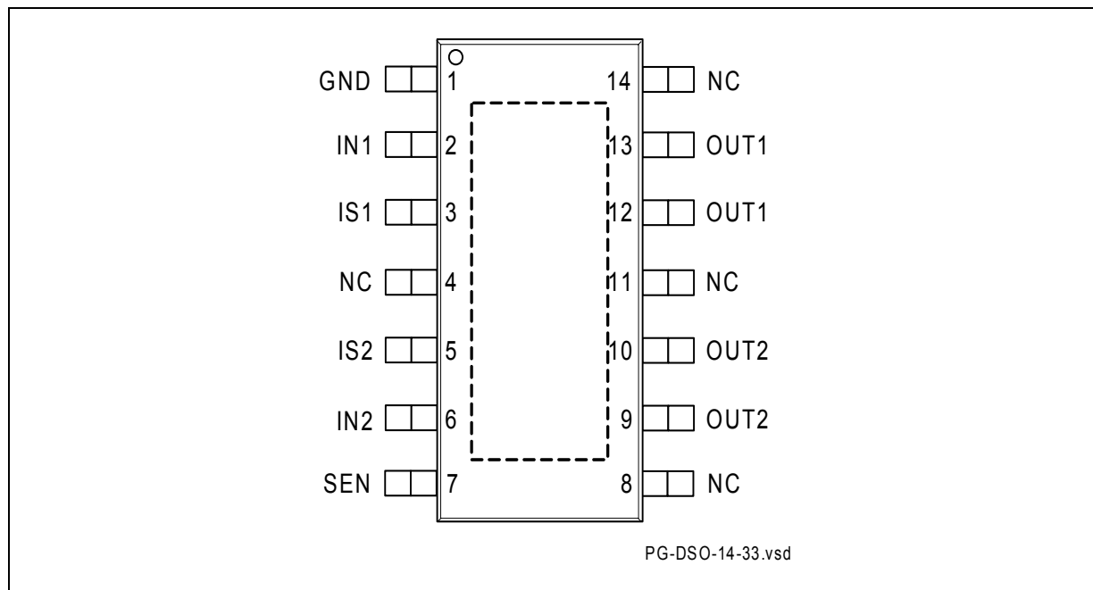
Figure 3 Pin Configuration PG-DSO-14-33
