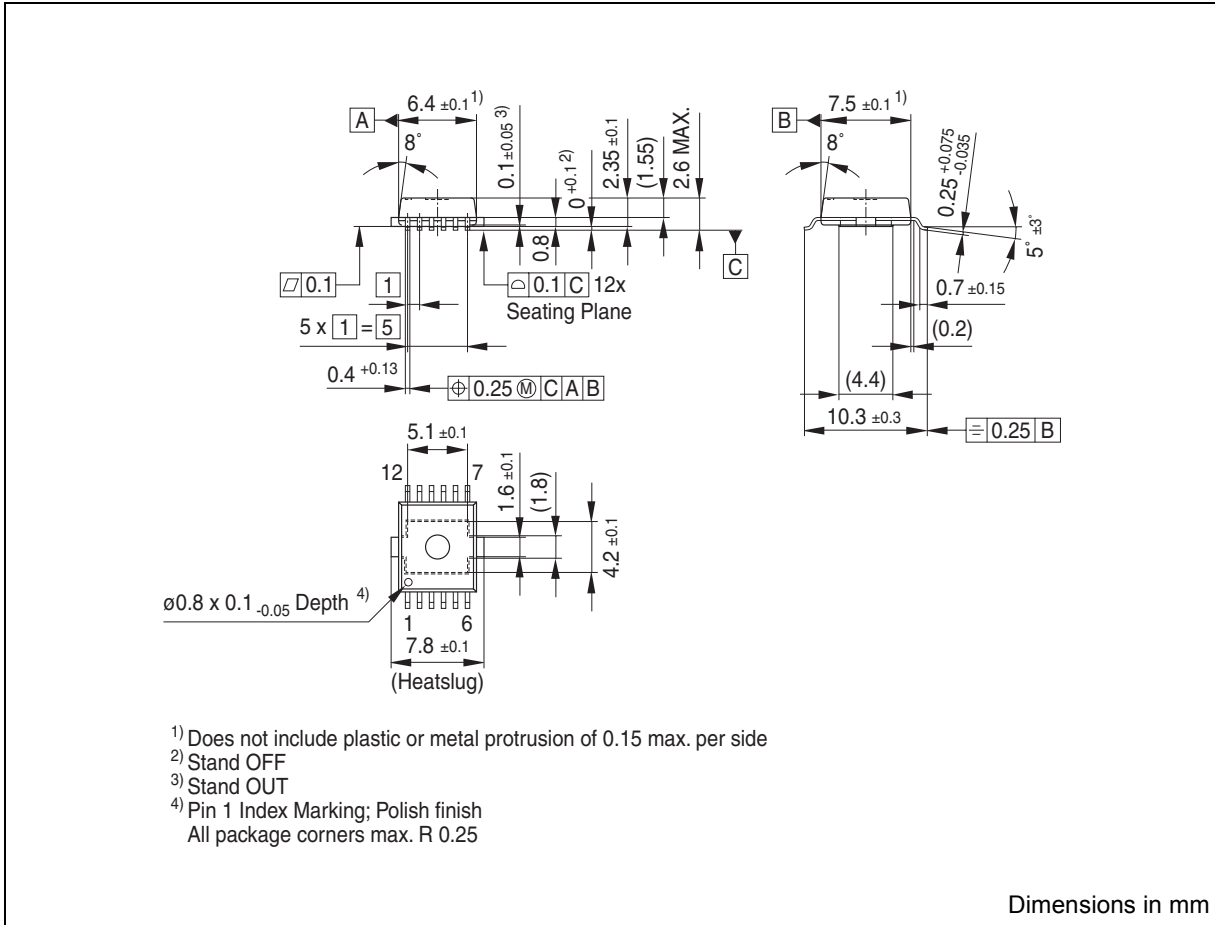
Figure 19 P-DSO-12-2 (Plastic Dual Small Outline Package)
