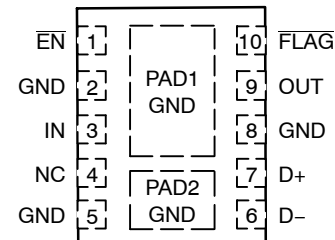
NCP362B Version (D+/- ESD low cap + OVP/OCP)
