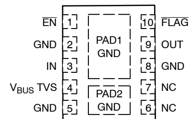
NCP362A Version ( V_{BUS} TVS + OVP/OCP)
