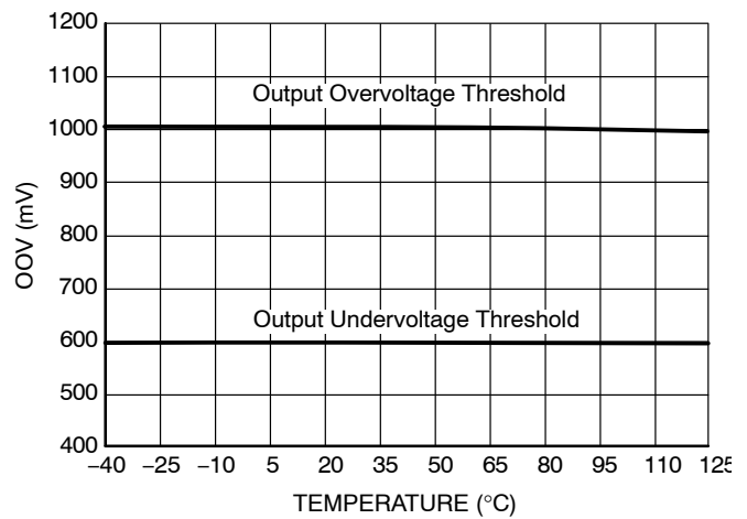
Figure 14. Output Protection vs Temperature
