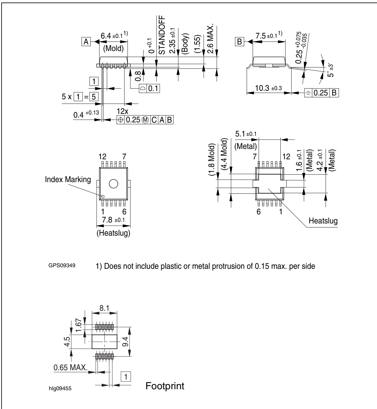
Figure 4 P-DSO-12-4 (Plastic Dual Small Outline)
