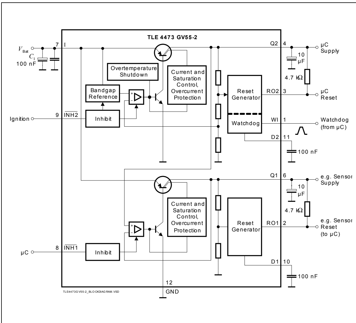
Figure 2 Block Diagram with Typical External Components
