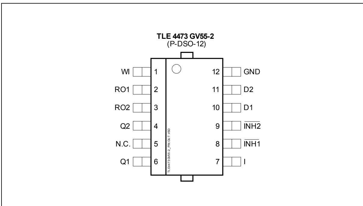
Figure 3 Pin Configuration (top view)
