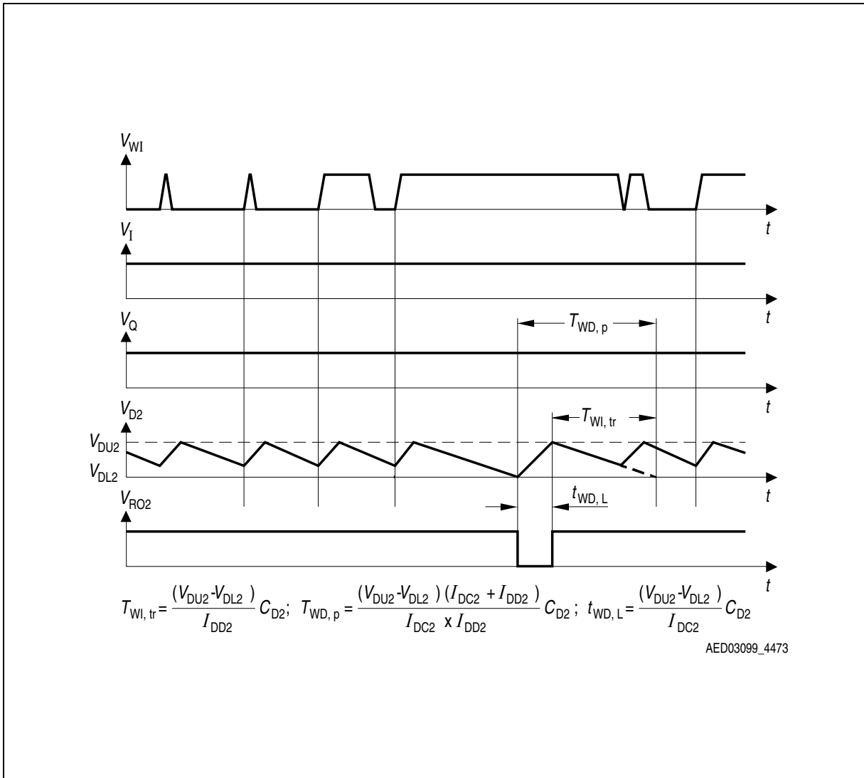
Figure 1 Watchdog Timing Schedule
