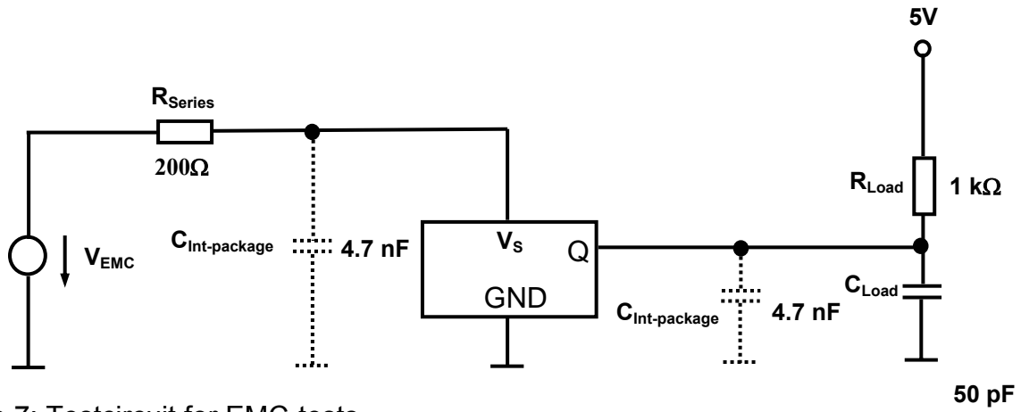
Figure 7: Testcircuit for EMC-tests
