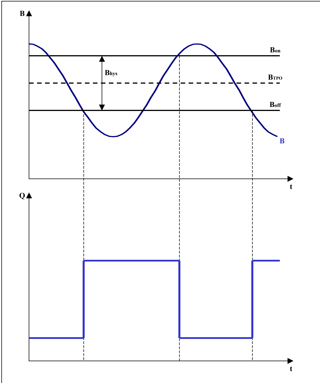
Fig. 1: Visible hysteresis (Initial mode, unprogrammed IC)
