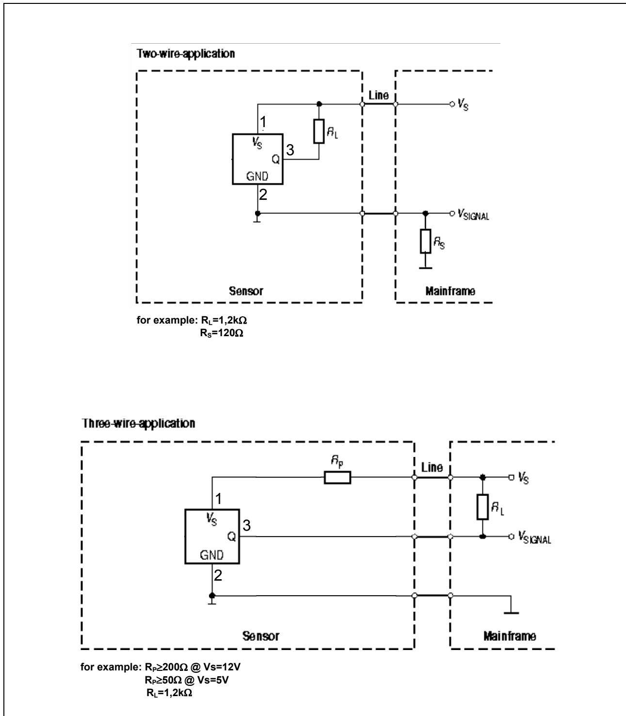
Figure 6 Application Circuits TLE4982C
