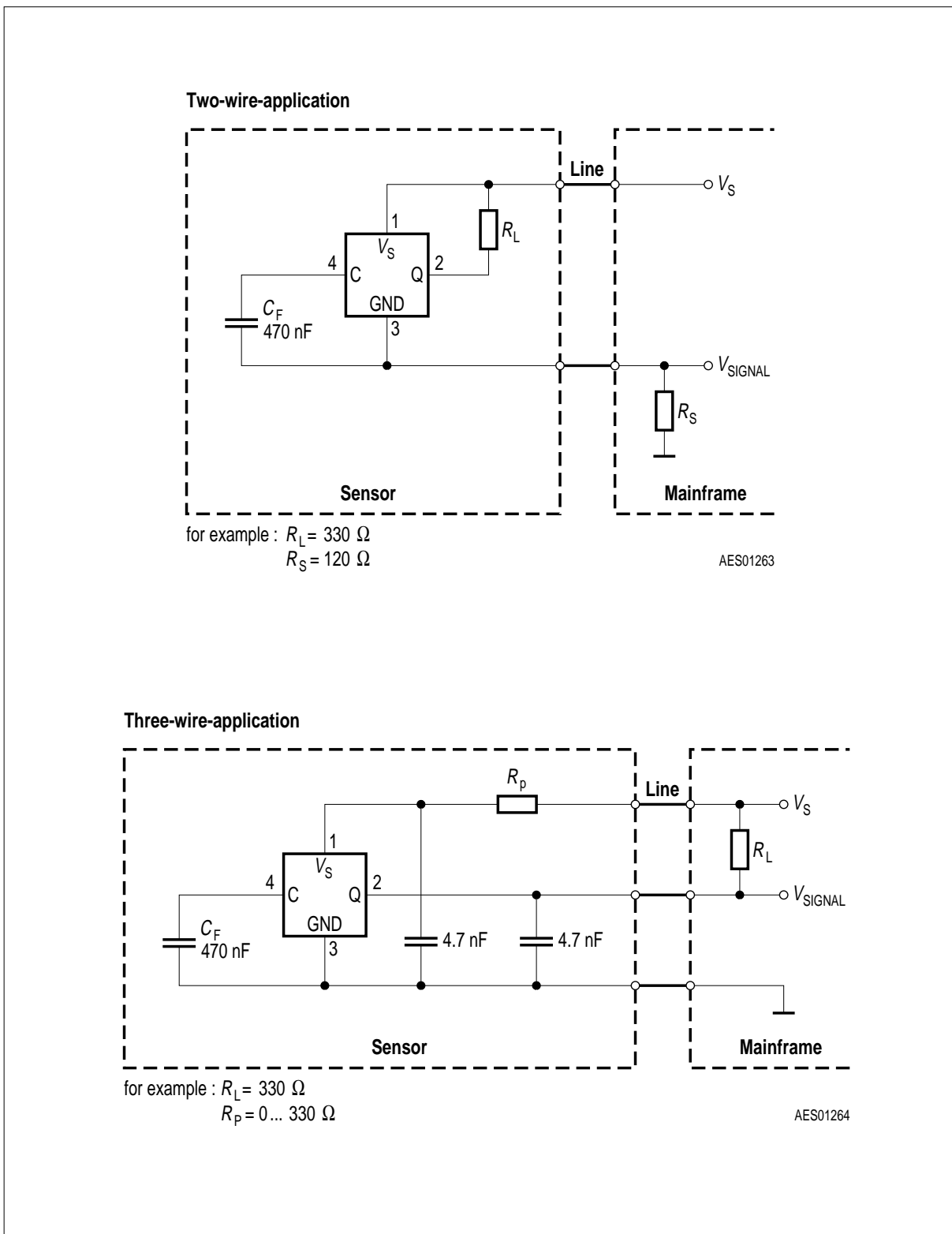
Figure 9 Application Circuits
