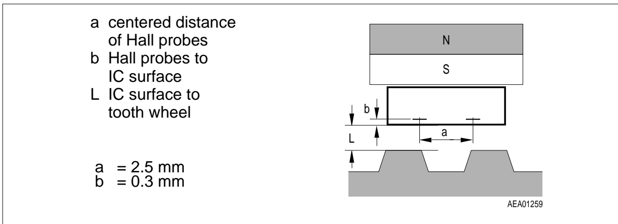
Figure 5 Sensor Spacing
