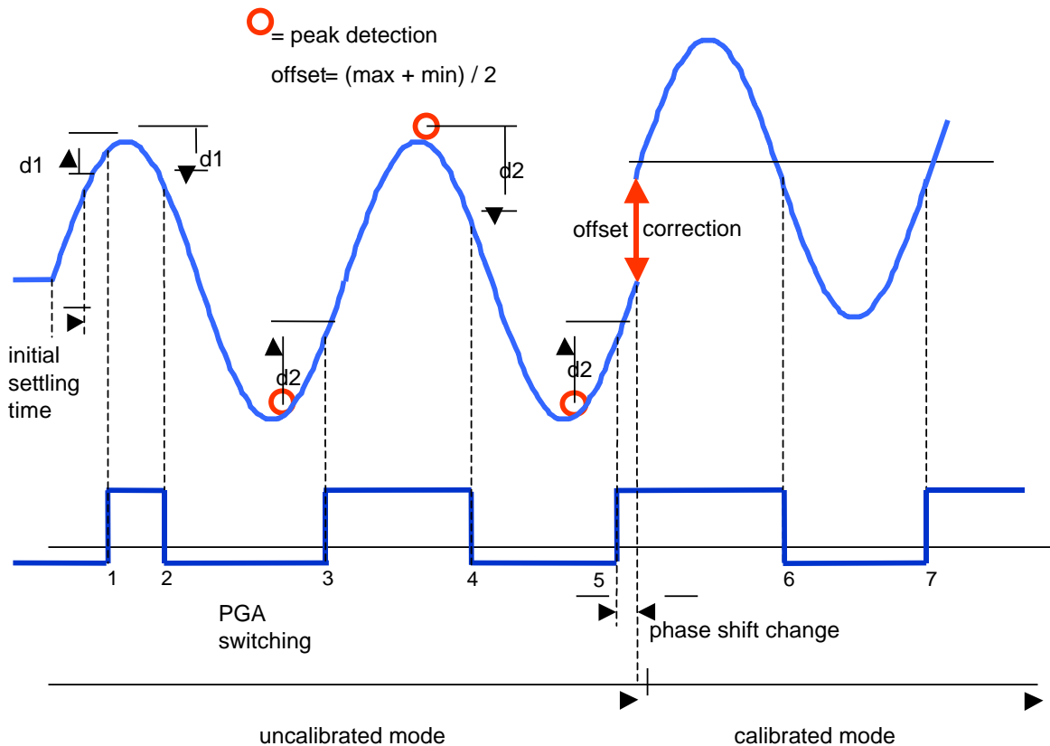
Fig. 1: example for startup behaviour
