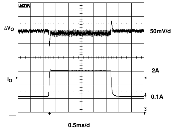
FIGURE 12. TRANSIENT RESPONSE
