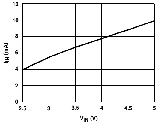
FIGURE 6. NO LOAD INPUT CURRENT
