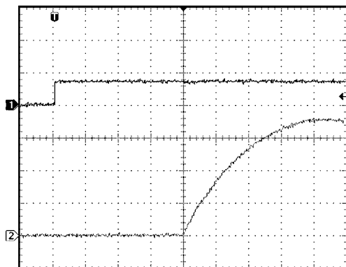
1.8V Mode Startup, Load = 300mA
