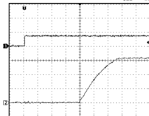
1.6V Mode Startup, Load = 300mA, V_{SEL} = V_{IN}
