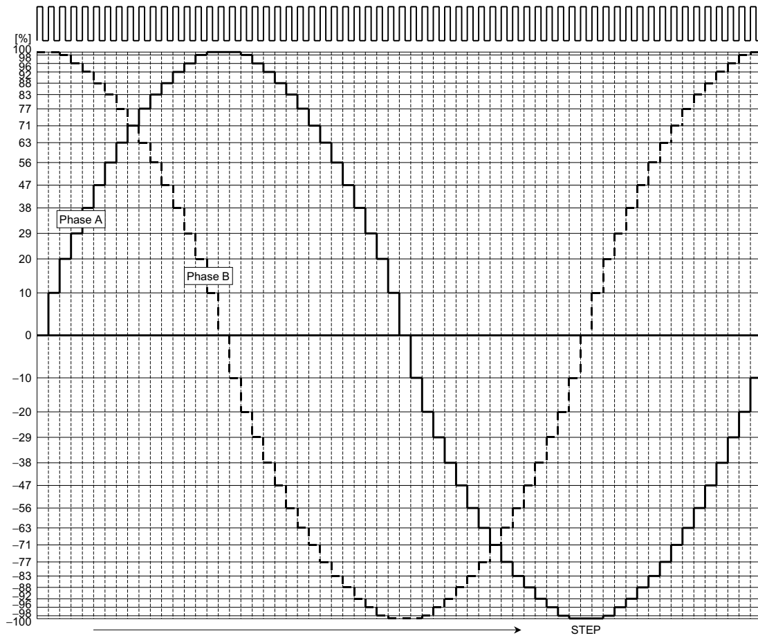
(8) 4W1-2 Phase Excitation mode
