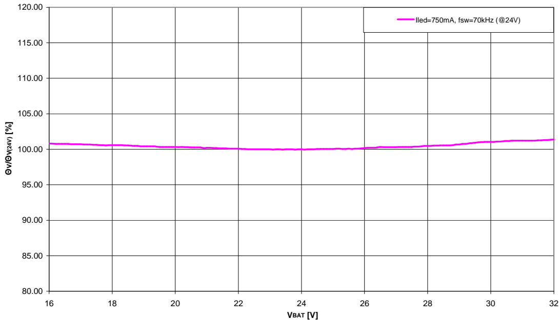
MLX10803 Normalized luminous flux \Phi_V/\Phi_{V(24V)} vs. supply voltage \Phi_V/\Phi_{V(24V)}=f(V_{BAT})
