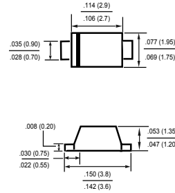
Dimensions in inches and (millimeters)
