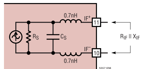
Figure 8. IF Output Small-Signal Model
