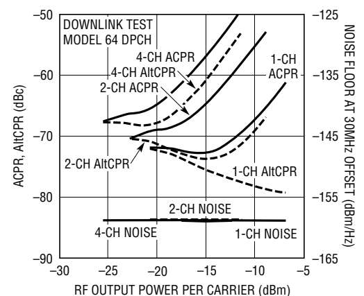
W-CDMA ACPR, A1cPR and Noise vs RF Output Power at 2.14GHz for 1, 2 and 4 Channels
