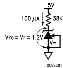
FIGURE 3. 1.2V Reference
