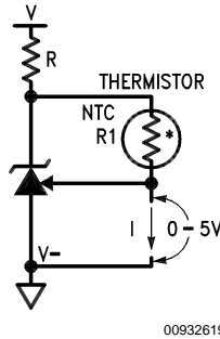
FIGURE 11. Negative-TC Current Source
