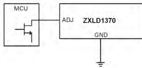
Figure 30: PWM dimming from MCU
