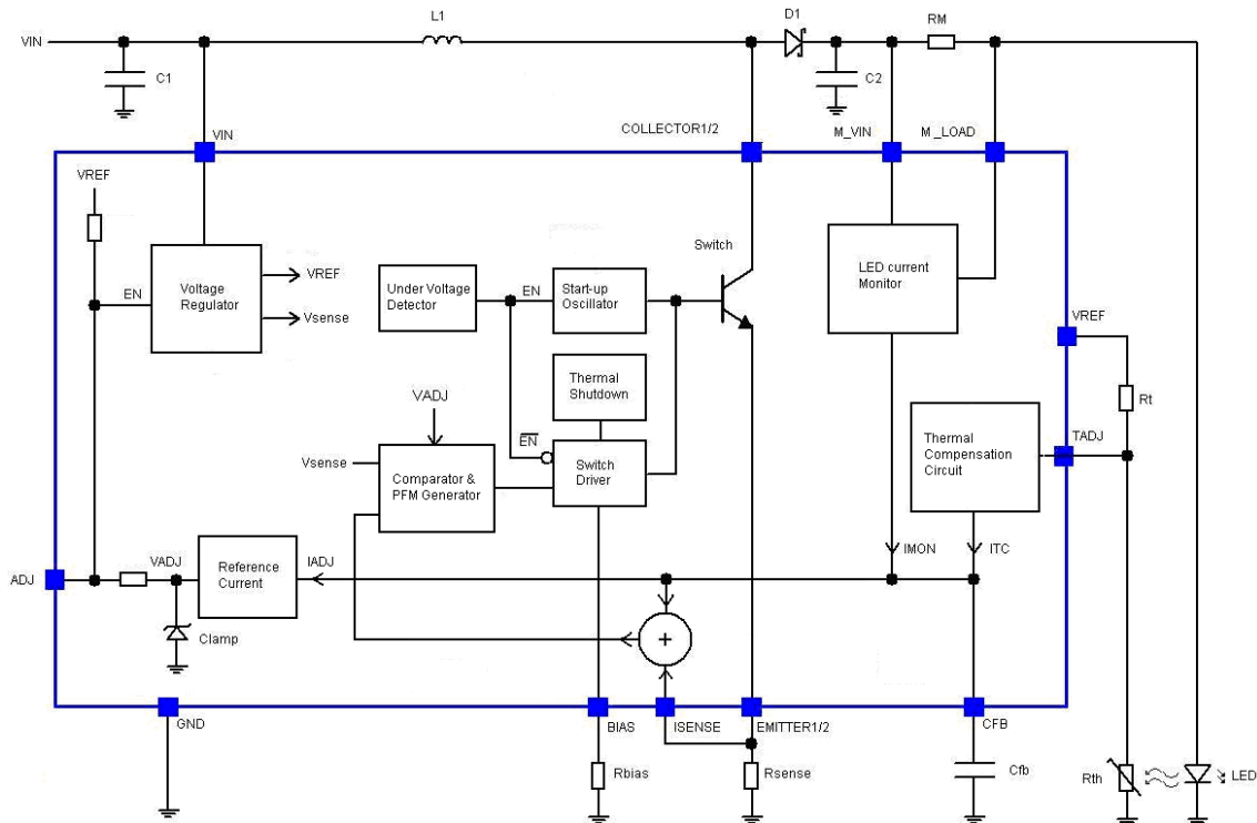
ZXLD1321 Block Diagram (showing external components)
