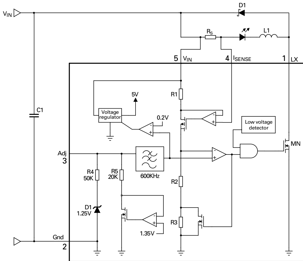
Figure 1 Block diagram
