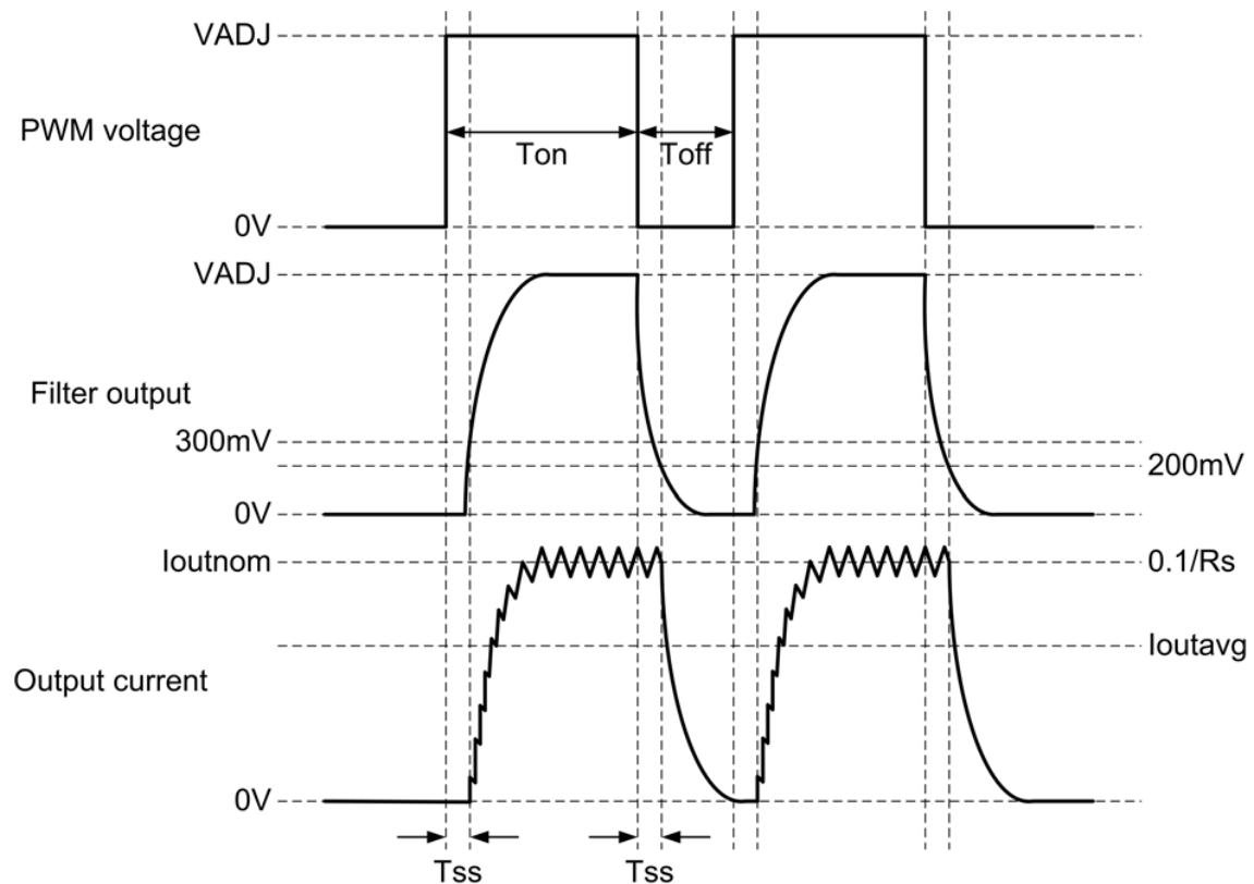
Figure 4 Low frequency PWM operating waveforms
