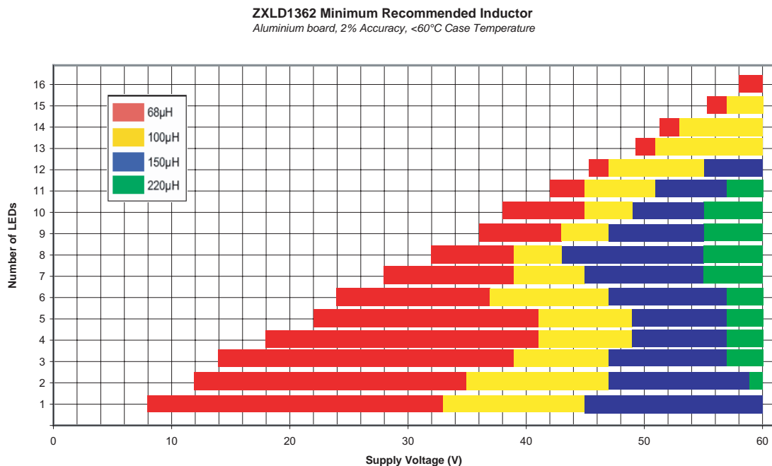
Figure 3 ZXLD1362 Minimum recommended Inductor
