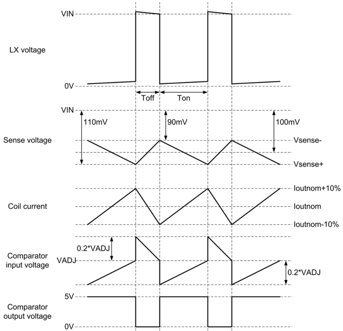
Figure 2 Theoretical operating waveforms
