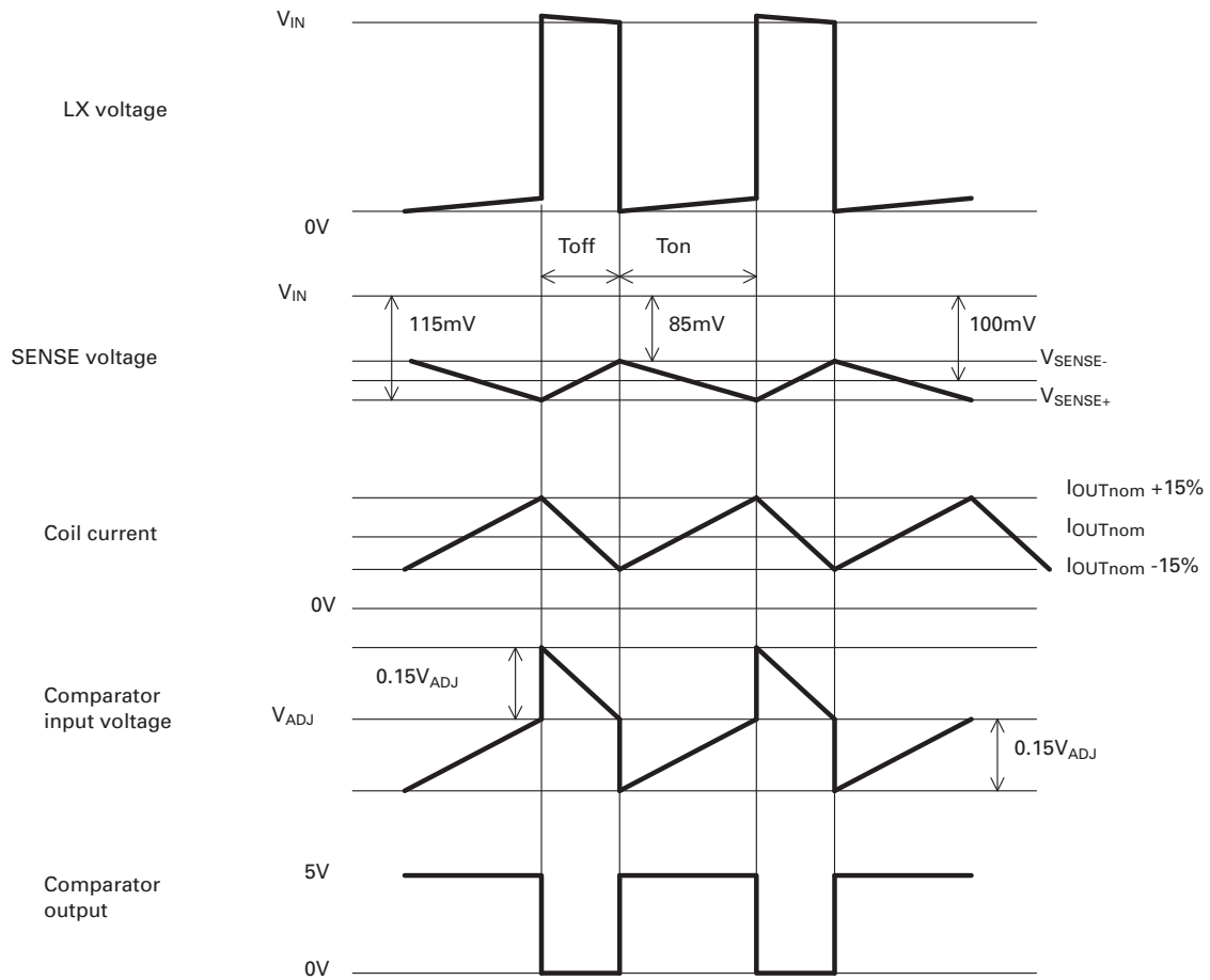
Figure 1 - Operating waveforms
