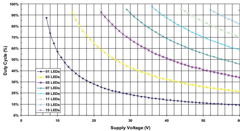
ZXLD1366 Duty Cycle L=220 \mu H
