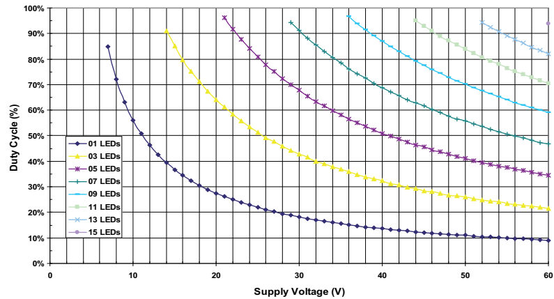
ZXLD1366 Duty Cycle L=68μH
