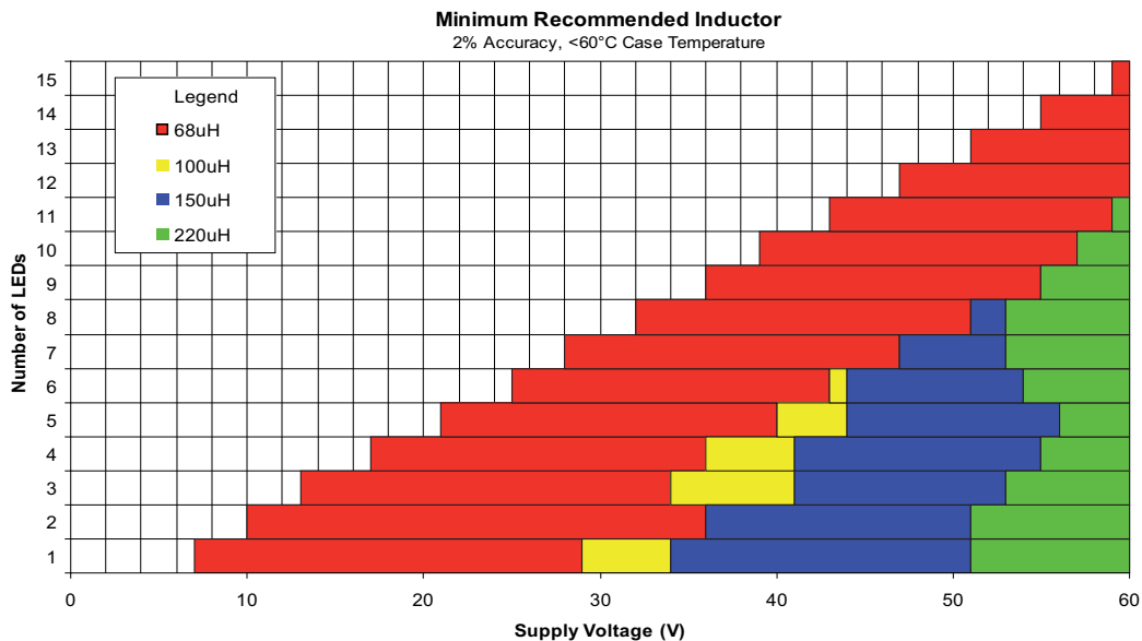
Figure 3 ZXLD1366 Minimum recommended inductor (TSOT)
