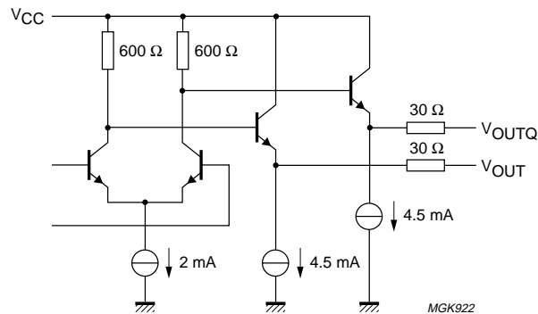
Fig.3 Data output buffer.
