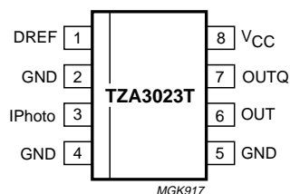
Fig.2 Pin configuration.
