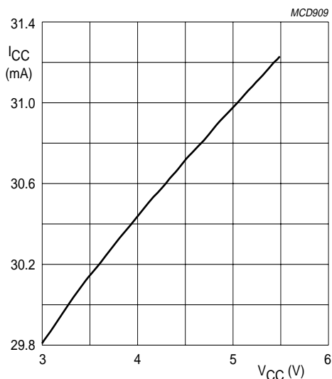
Fig.9 Supply current as a function of the supply voltage.
